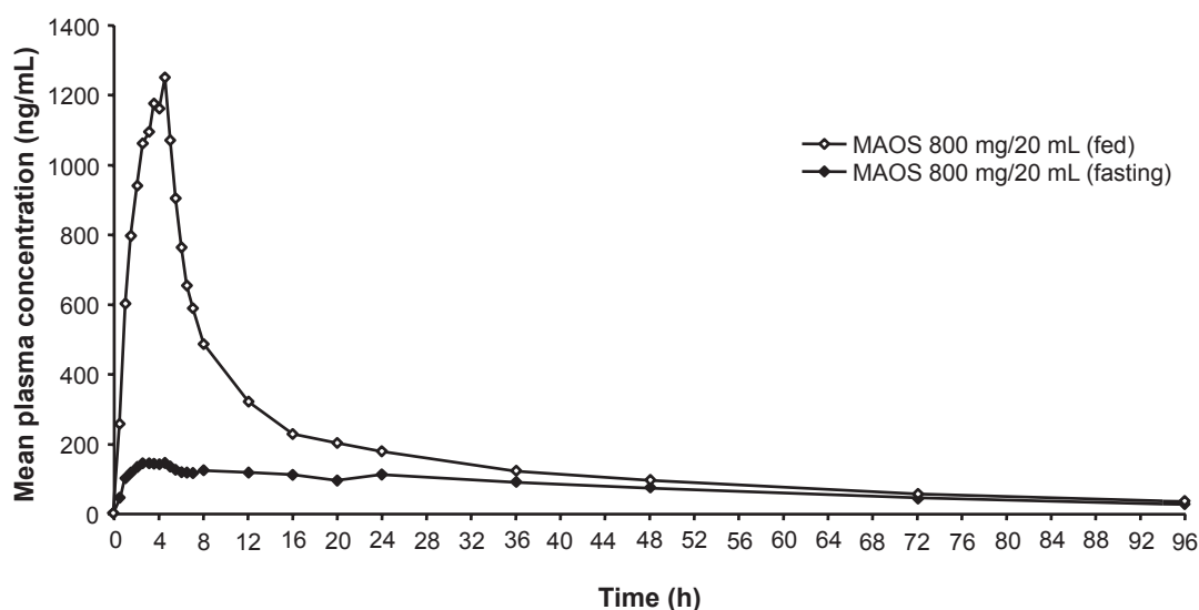
Figure 3 Mean plasma concentration profile a for a micronized formulation of megestrol acetate oral suspension (MAOS) 800 mg/20 mL in fed and fasting states. Data from Study 2, MAOS in fed (N = 32) subjects, and Study 3, MAOS in fasting (N = 36) subjects.
