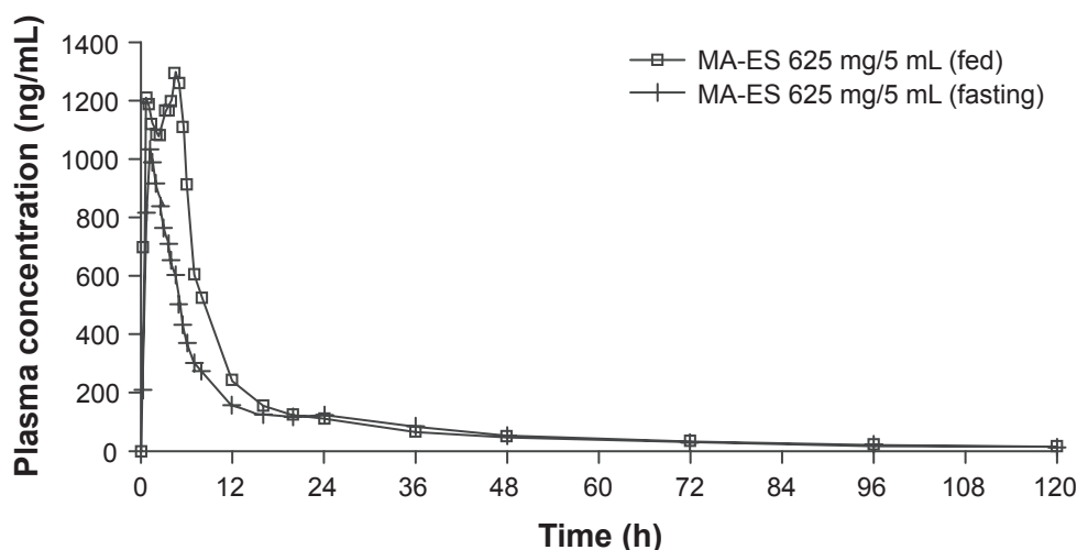
Figure 2 Mean plasma concentration profile a for a nanocrystal dispersion of megestrol acetate (MA-ES) 625 mg/5 mL in fed and fasting states (N = 23). Data from Study 1.
