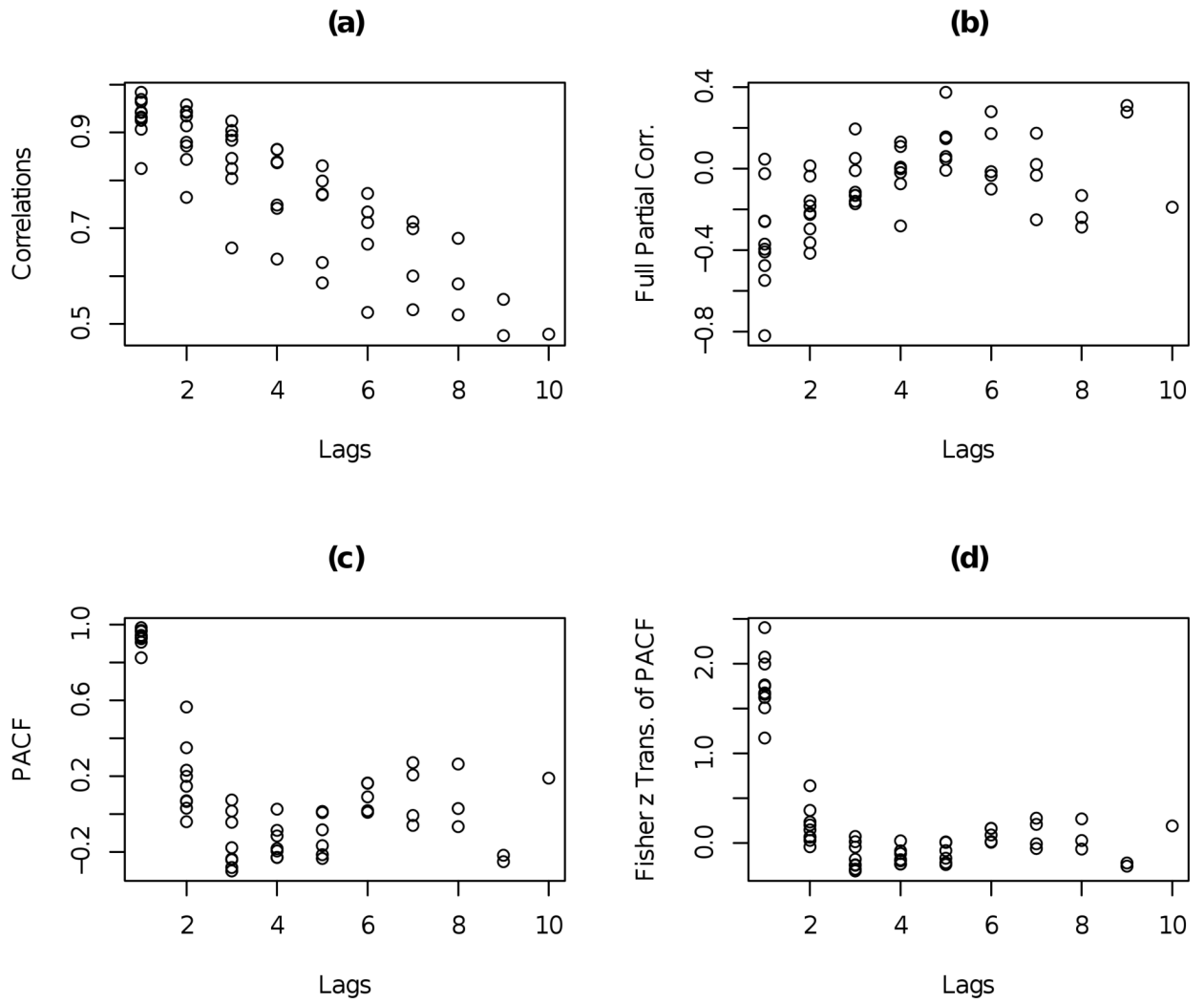
Figure 1. (a) Generalized sample correlogram for the cattle data, (b) Generalized inverse correlogram, (c) Generalized partial correlogram, (d) Plot of Fisher z transform of the PACF.
