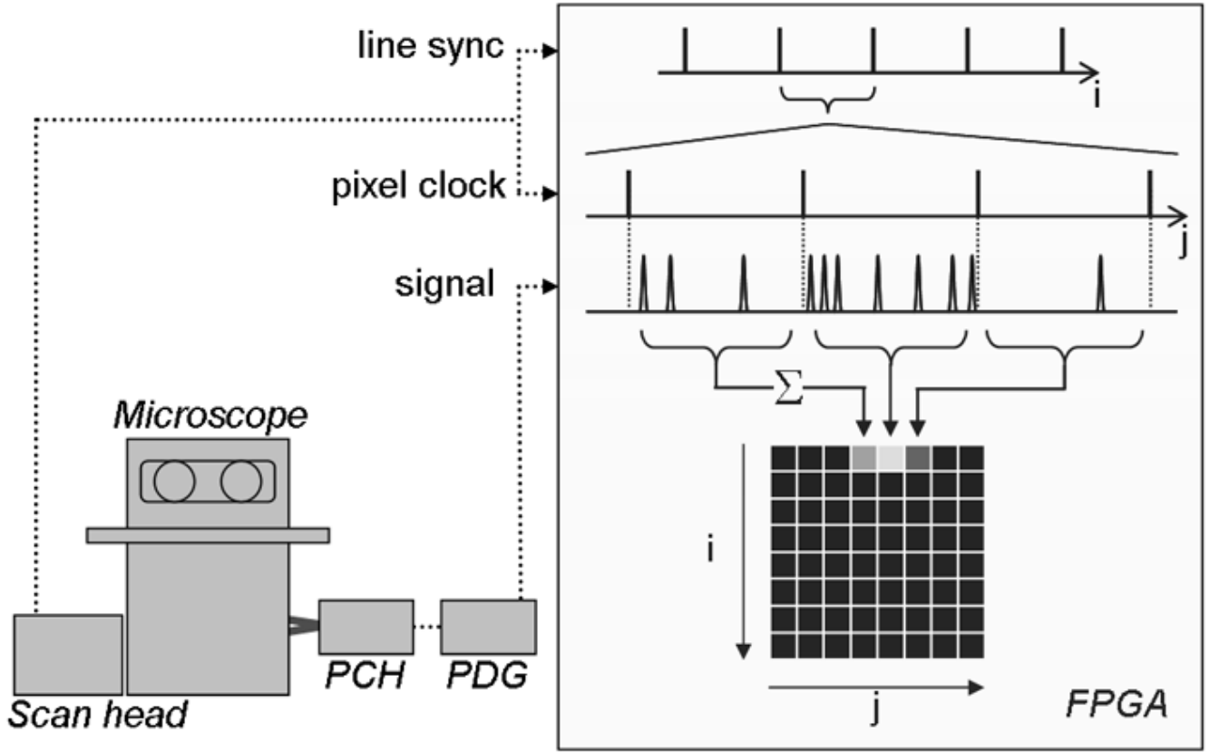
Figure 1. Schematic of the single-photon counting detector system. The photon counting head (PCH) relays the single photon event TTL pulse via the pulse delay generator (PDG) to the field programmable gate array (FPGA). Line synchronization (sync') and pixel clock signals from the confocal scan head are also sent to the FPGA. On the FPGA, after every pixel clock tick, the photon event pulses are counted until the following pixel clock tick. This count ( \Sigma ) is then input into the pre-allocated memory array, at a position defined by the line sync' and pixel clock signal ( i,j ).
