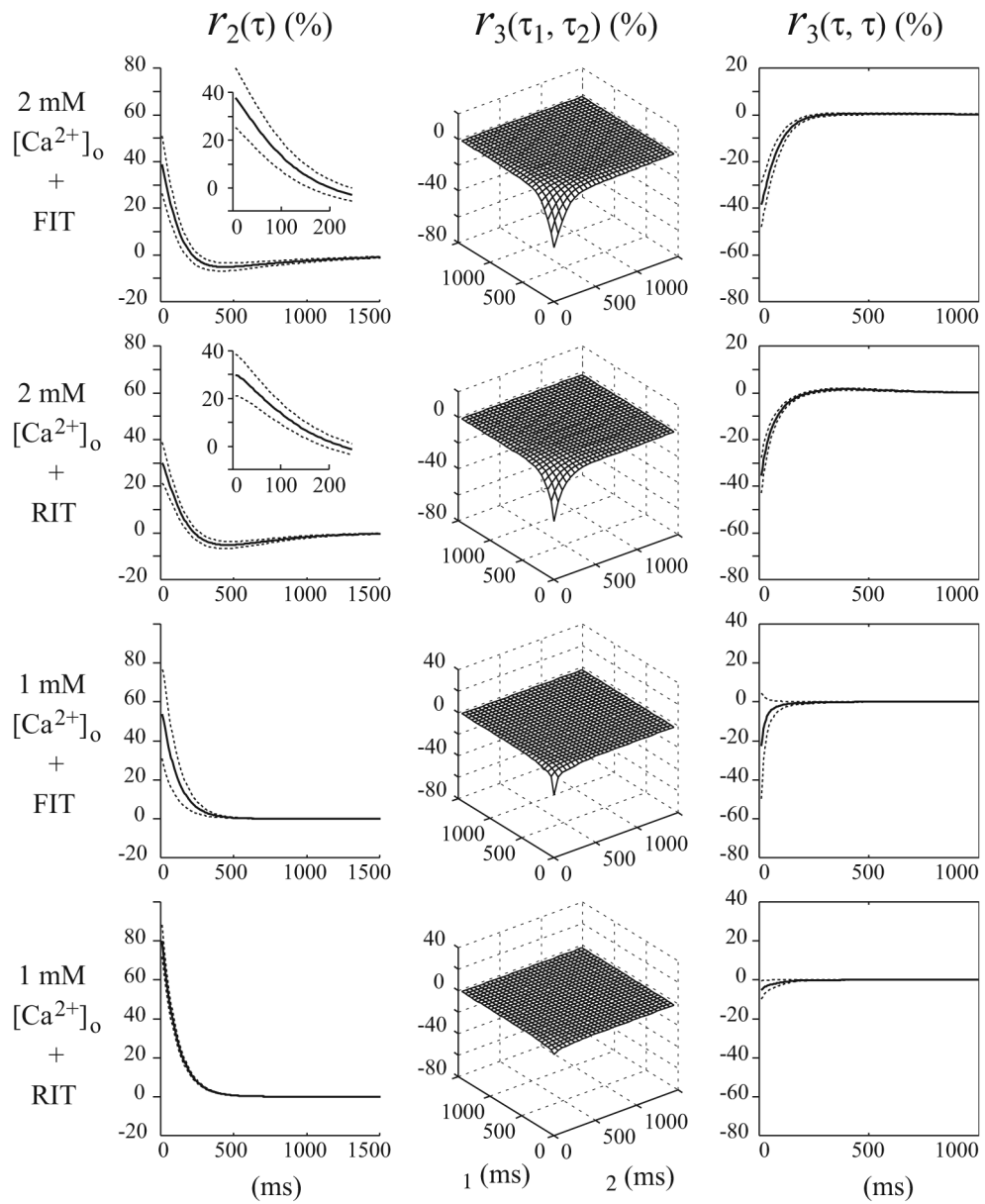
Fig. 7. RDs of the 3rd-order Poisson–Volterra models obtained by use of the simulated input–output data of the parametric FD models with parameters estimated from the fixed-interval and random-interval datasets under the two calcium conditions
