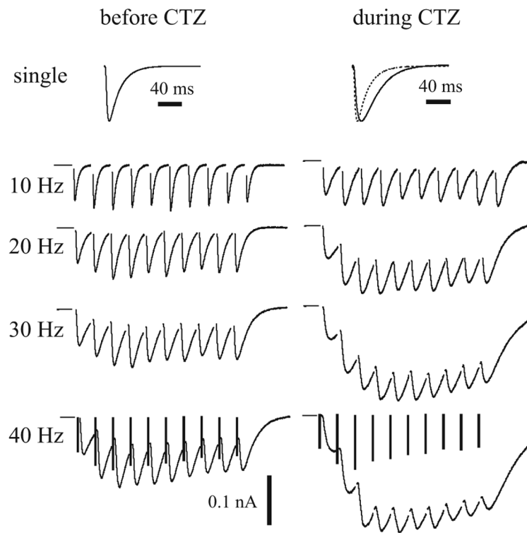
Fig. 5. Representative fixed-interval EPSC trains before and during CTZ application. The bars in bottom row denote the deconvolved EPSC amplitudes, which are not significantly affected by CTZ despite the dramatic changes in the corresponding EPSC waveforms
