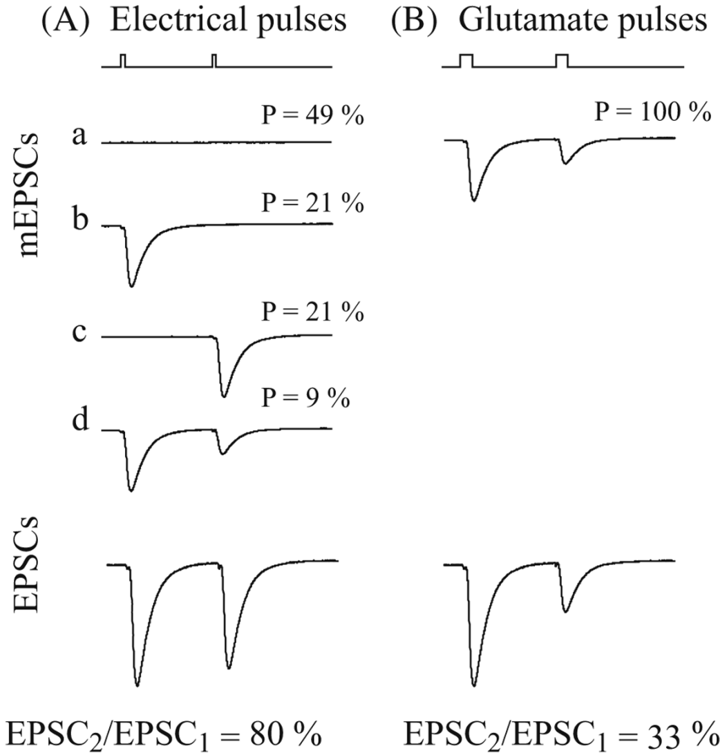
Fig. 10. Simulated experiment showing that the paired-pulse depression caused by AMPA receptor desensitization is attenuated by the probabilistic releases. (A) mEPSCs and EPSCs elicited by pairs of electrical pulses. a , b , c and d are the four possible patterns of mEPSCs. Desensitization only occurs in d . (B) mEPSCs and EPSCs elicited by pairs of glutamate pulses. Desensitization always occurs. In both (A) and (B) , the second EPSCs were normalized by the amplitude of the first EPSC. Note the different levels of depression caused by desensitization
