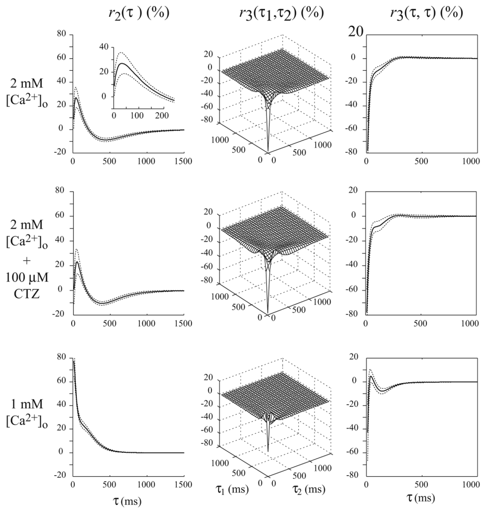
Fig. 4. The 2 nd and 3 rd order response descriptors (RDs), r_2 and r_3 , of the 3 rd -order Poisson–Volterra models of the SC synaptic dynamics obtained from broadband experimental data for different [Ca^{2+}]_o and CTZ conditions. Top row inset: the r_2 values for short inter-impulse intervals
