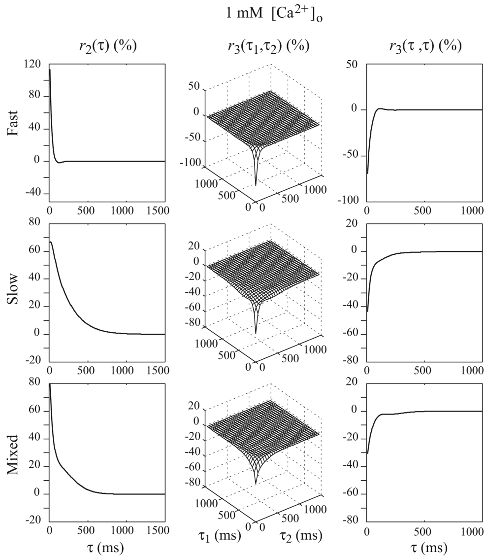
Fig. 9. The computed 2 nd and 3 rd order RDs of the parametric double-process FD model of the SC synapse with parameters estimated from the random-interval input–output experimental data under 1 mM [Ca^{2+}]_o condition
