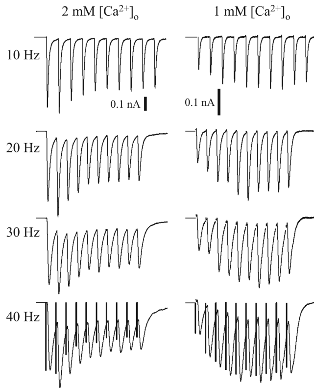
Fig. 3. Representative fixed-interval EPSC trains with four different frequencies and under two [Ca^{2+}]_o conditions. Each EPSC train is the average of 16 sweeps. Bars in bottom row are the deconvolved EPSC amplitudes representing the estimated transmitter release. Note the difference between the deconvolved EPSC amplitudes and the peak EPSC amplitudes due to the temporal summations in the EPSC train
