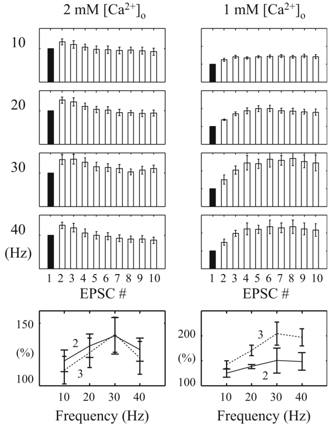
Fig. 2. Fixed-interval EPSC trains elicited with four different frequencies (10, 20, 30, 40 Hz) and under two different [Ca^{2+}]_o conditions. Under 2 mM [Ca^{2+}]_o condition, the EPSC peaks at the 2 nd response and then declines; while under 1 mM [Ca^{2+}]_o condition, the EPSC peaks later and attains almost a steady-state value. Note that the second to the tenth EPSCs (white bars) were normalized with the first EPSC (black bar). Bottom row: the 2 nd (solid lines) and 3 rd (dashed lines) responses as a percentage of the 1 st response
