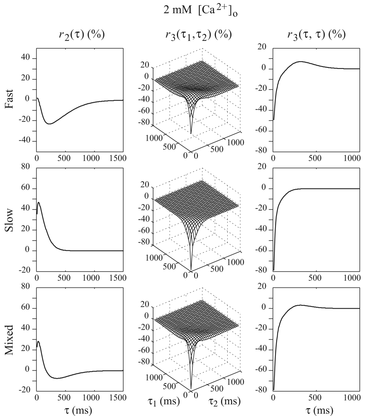
Fig. 8. The computed 2 nd and 3 rd order RDs of the parametric double-process FD model of the SC synapse with parameters estimated from the random-interval input–output experimental data under 2 mM [Ca^{2+}]_o condition
