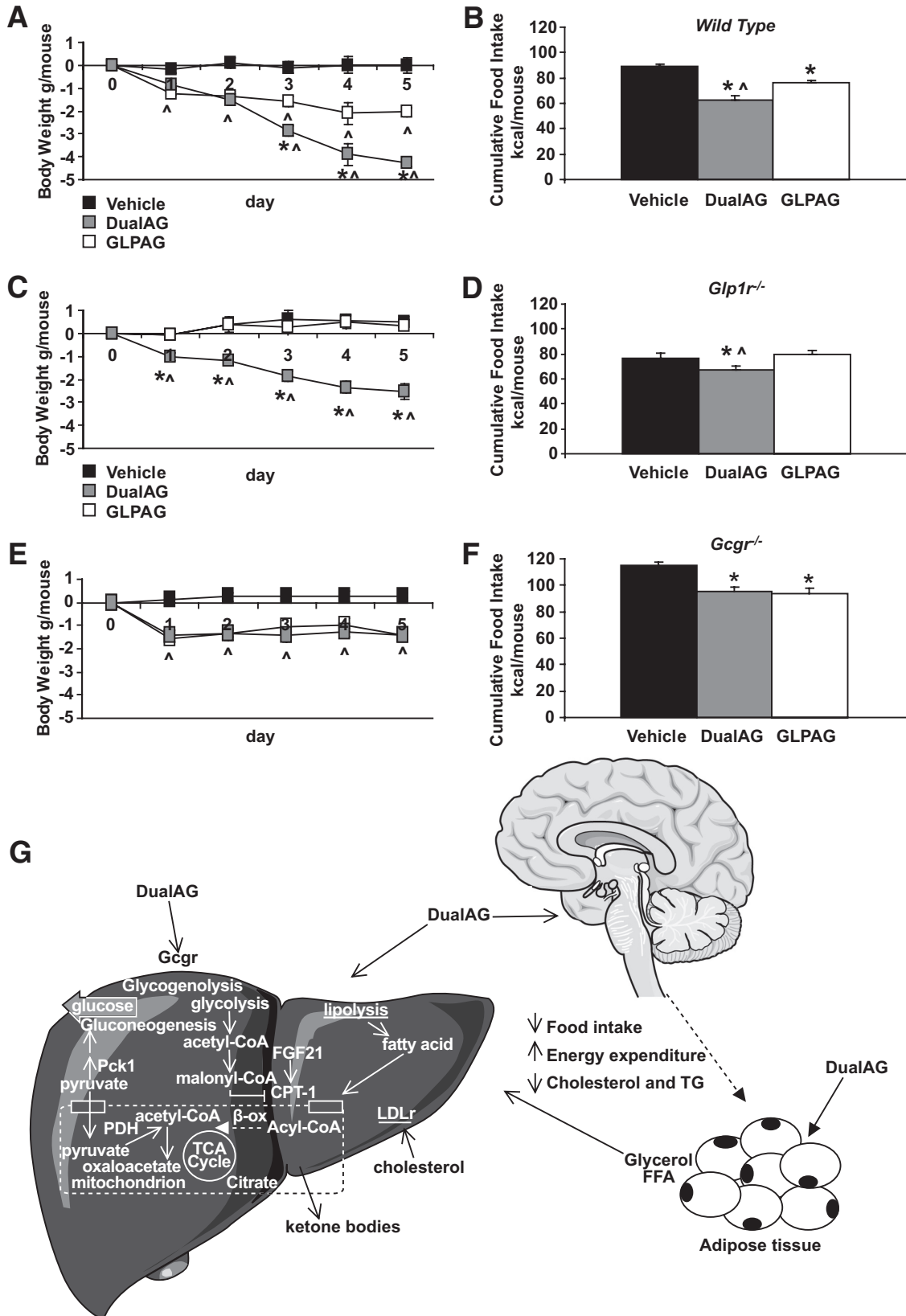
FIG. 5. DualAG lowers body weight and food intake via activation of GLP1R and GCGR. Effect of repeated injections of DualAG or GLPAG on cumulative food intake and body weight in wild-type ( A and B ), Glp1r -/- ( C and D ), and Gcgr -/- ( E and F ) mice. The antiobesity effects of DualAG are attenuated but not ablated in either receptor knockout mouse. G : Proposed mechanism of action of DualAG. In addition to the known effects associated with GLP1R activation, hepatic GCGR activation increases liver glucose production and stimulates FAO. The acetyl-CoA generated by \beta -oxidation challenges the processing capacity of the tricarboxylic acid (TCA) cycle and is used in the biosynthesis of ketone bodies. Consistent with the decrease in plasma cholesterol, animals treated with DualAG showed a robust upregulation of liver LDLr expression. In the adipose tissue, pharmacological activation of GCGR and GLP1R may stimulate hydrolysis of triglycerides (TG). Upregulation of liver Fgf21 in animals treated with DualAG may contribute to stimulation of FAO and ketogenesis. * P < 0.05 DualAG and GLPAG versus vehicle; ^ P < 0.05 DualAG versus GLPAG. FFA, free fatty acid.
