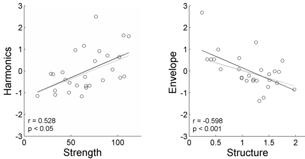
Figure 4. Relationships between DPOAE measures and their predictors. (A) DPOAE Strength is positively related to its strongest predictor, Harmonics , while (B) Structure is negatively related to its strongest predictor, Envelope Boundary . All brainstem composite measures are plotted as Z-scores. Black lines (and reported statistics) are regressions using all data points, grey lines are the regressions omitting individuals with Z > 2 .
