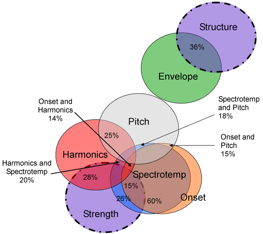
Figure 3. Venn diagram of the relationships between composite sABR and DPOAE measures. sABR circles are solid; DPOAE circles are dashed. The percentage overlap between the variables ( R^2 ; bivariate relationships) is marked. While all measures are in some minor way related, and all circles in the figure should be touching, any overlap not reported was less than 0.5%. Spectrotemporal was shortened to Spectrotemp for space constraint reasons. Note that only a weak relationship was observed between the two DPOAE composite measures, Strength and Structure ( R^2 = 0.0025 ).
