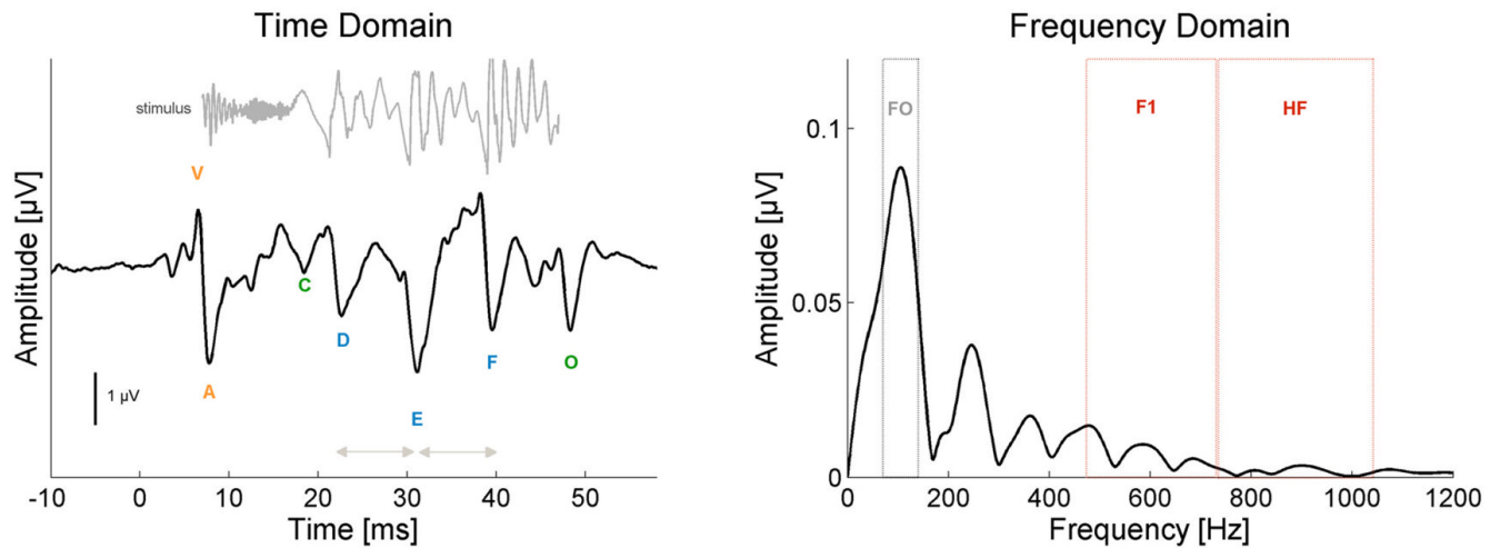
Figure 2. Schematic of the brainstem response to the speech syllable [da] in the time (left) and frequency (right) domains. The time domain waveform of the stimulus is plotted in gray above sABR waveform. The stimulus is time-shifted 8 ms in order to facilitate its visual comparison with the response by accounting for the neural conduction lag. Onset measures (V, A latencies) are labeled in orange. Spectrotemporal (D, E, F latencies) elements are labeled in blue. Envelope Boundary measures (C, O latencies) are labeled in green. Pitch measures ( F_0 amplitude, E–D, F–E inter-peak latencies) are labeled in grey and Harmonic measures ( F_1 , HF amplitudes) are labeled in red.
