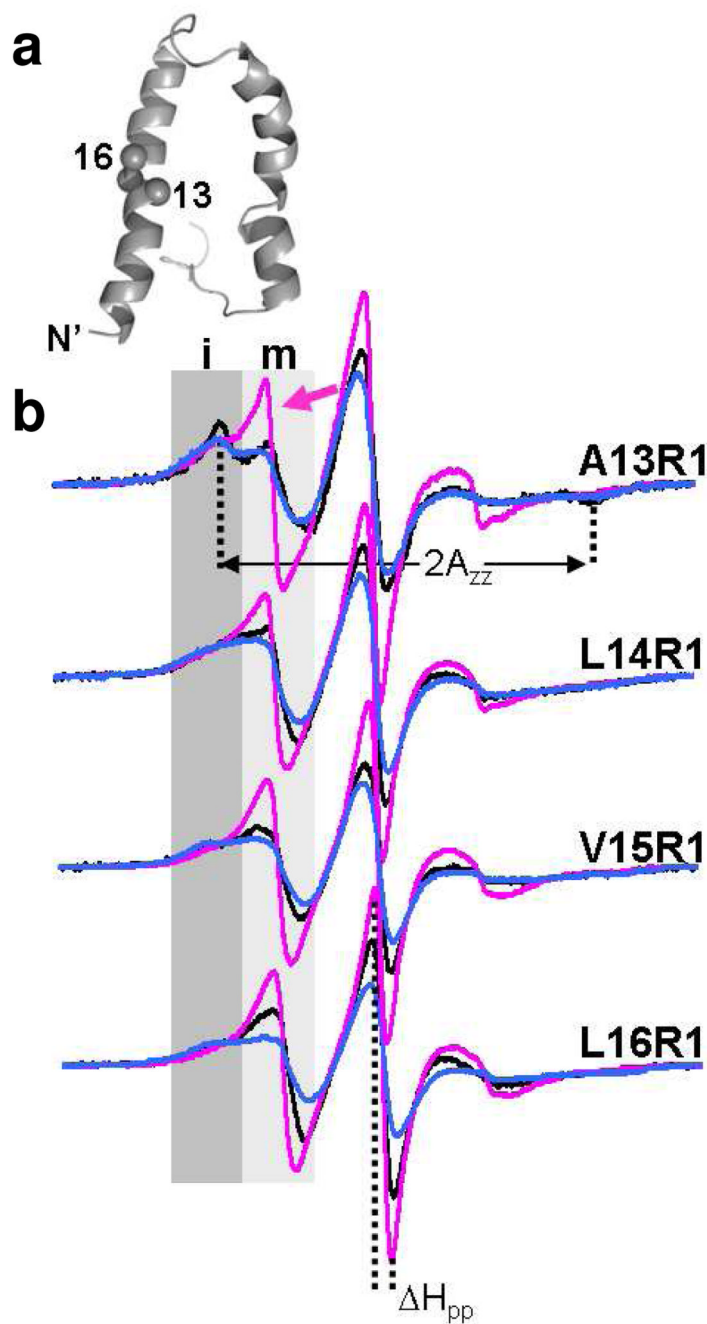
Figure 2. Effects of the detergent on protein structure and dynamics. (a) A ribbon model of TM0026 with the spin labeled residues A13 – L16 represented by spheres (see Methods section for modeling). (b) The EPR spectra of R1 at residues A13 – L16 in DM, DDM, and FC-10 are shown and colored according to the labels in Figure 1. Spectral intensities in regions labeled i (dark gray) and m (light gray) identify relatively immobile and mobile components, respectively. The arrow indicates a dynamic population observed in FC-10. The semi-quantitative measurements, \Delta H_{pp} and 2A_{zz} , are indicated.
