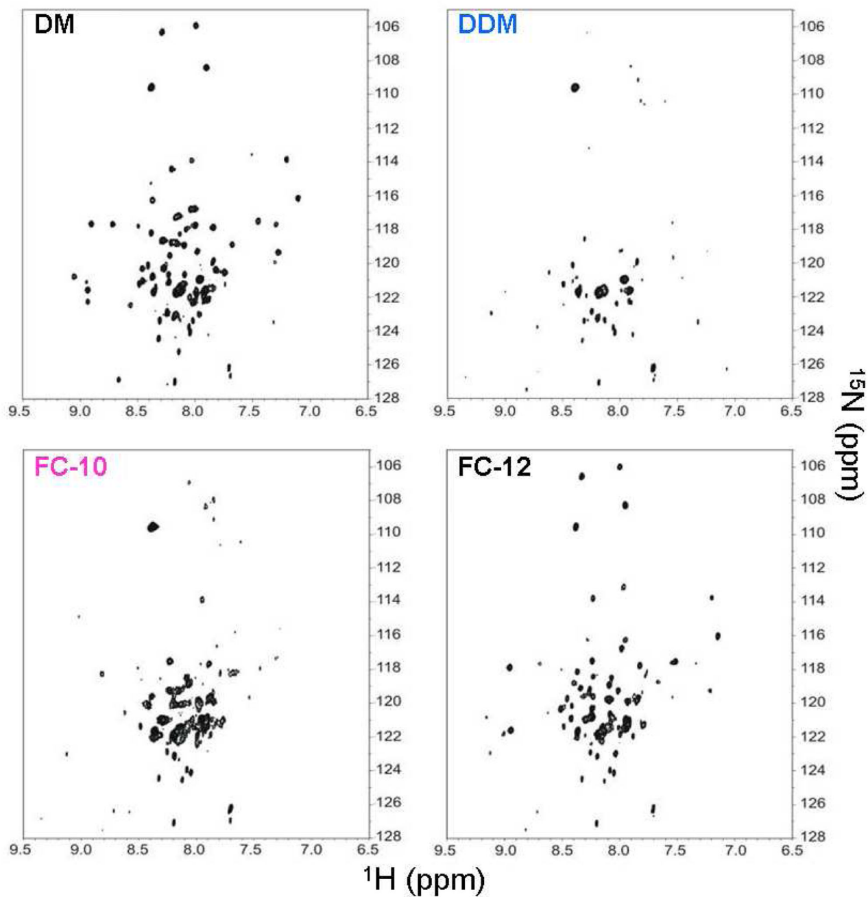
Figure 1. Soluble protein-detergent complexes differ in conformational heterogeneity. The NMR ^{15}\text{N} , ^1\text{H} -TROSY spectra of ^2\text{H} , ^{15}\text{N} -labeled TM0026 in DM, DDM, FC-10, and FC-12 are shown.
