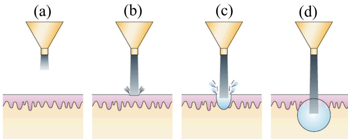
Figure 1. Schematic of drug delivery using liquid jet injector (to be printed after permission from (Mitragotri 2006)) (a) Formation of liquid jet (b) Initiation of hole formation due to impact of jet on skin surface (c) Development of hole inside skin with progress of injection (d) Deposition of drug at the end of hole in a near spherical or hemispherical pattern (spherical pattern shown).
