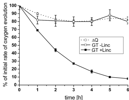
FIG. 2. Photoinhibition analyses of the Synechocystis sp. strain PCC 6803 GT and the \Delta Q quadruple mutant. Cells at a Chl a concentration of 20 \mu\text{g ml}^{-1} were treated with high light ( 1,200 \mu\text{E m}^{-2} \text{s}^{-1} ) at 29^\circ\text{C} over a period of 6 hours. Oxygen evolution of whole cells was assessed for the Synechocystis sp. strain PCC 6803 GT and the \Delta Q quadruple mutant strains in the presence or absence of 100 \mu\text{g ml}^{-1} lincomycin at the indicated time points in the presence of 2 mM DCBO and 1 mM \text{K}_3\text{Fe}(\text{CN})_6 using a Hansatech DW2 oxygen electrode (Hansatech Instruments Ltd., United Kingdom). Oxygen evolution rates (in \mu\text{mol} oxygen per mg of Chl a per h) were normalized (value at t = 0 was 100%) and plotted as a function of time. Error bars represent standard deviation from the means of three measurements. The initial, absolute rates of oxygen evolution for the respective strains were as follows: 324 ( \Delta Q without Linc), 316 (GT without Linc), and 350 (GT +Linc) (all in \mu\text{mol} oxygen per mg of Chl a per h).
