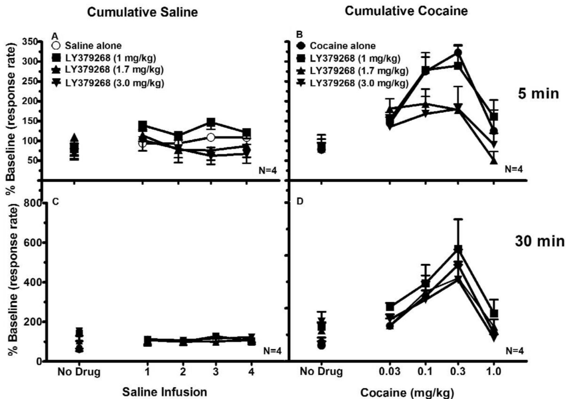
Figure 2. Cumulative infusions of saline did not significantly alter baseline rates of responding maintained by a fixed-interval schedule of stimulus termination in four squirrel monkeys (A). Cumulative doses of cocaine (0.03-1.0 mg/kg) produced a typical inverted-U shaped dose effect curve (B). Both 0.1 and 0.3 mg/kg cocaine produced significant increases in rates of responding. LY379268 (1.0-3.0 mg/kg) pretreatments did not significantly alter rates of responding maintained by a fixed-interval stimulus-termination schedule when repeated injections of saline were administered (A,C). However, a 5-min LY379268 pretreatment produced a downward shift of the cocaine dose effect curve (B). In contrast, a 30-min pretreatment time was ineffective in attenuating the behavioral-stimulant effects of cocaine (D). Abscissae: drug dose or saline infusion. Ordinates: rates of responding expressed as a percent of baseline control rates.
