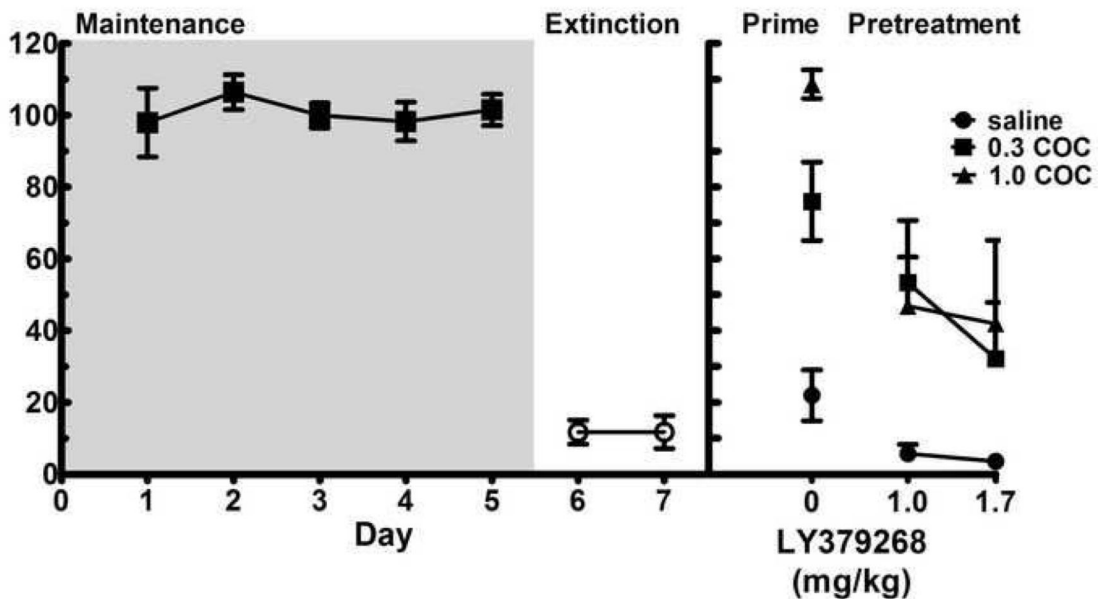
Figure 4. Cocaine self-administration was reliable during the maintenance phase, and extinguished readily in 2 sessions in four squirrel monkeys. Subsequently, non-contingent injections of cocaine (0.3 and 1.0 mg/kg) reinstated responding. LY379268 pretreatment demonstrated a strong trend toward significantly attenuating reinstatement of responding induced by the high dose (1.0 mg/kg) of cocaine. Abscissa: day of treatment and pretreatment dose of LY379268 prior to reinstatement tests. Ordinate: rates of responding expressed as a percent of baseline control rates.
