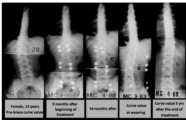
Figure 9 Example of the effectiveness of the derotation actions with inversion of proximal vertebrae rotation and curve doubling.
