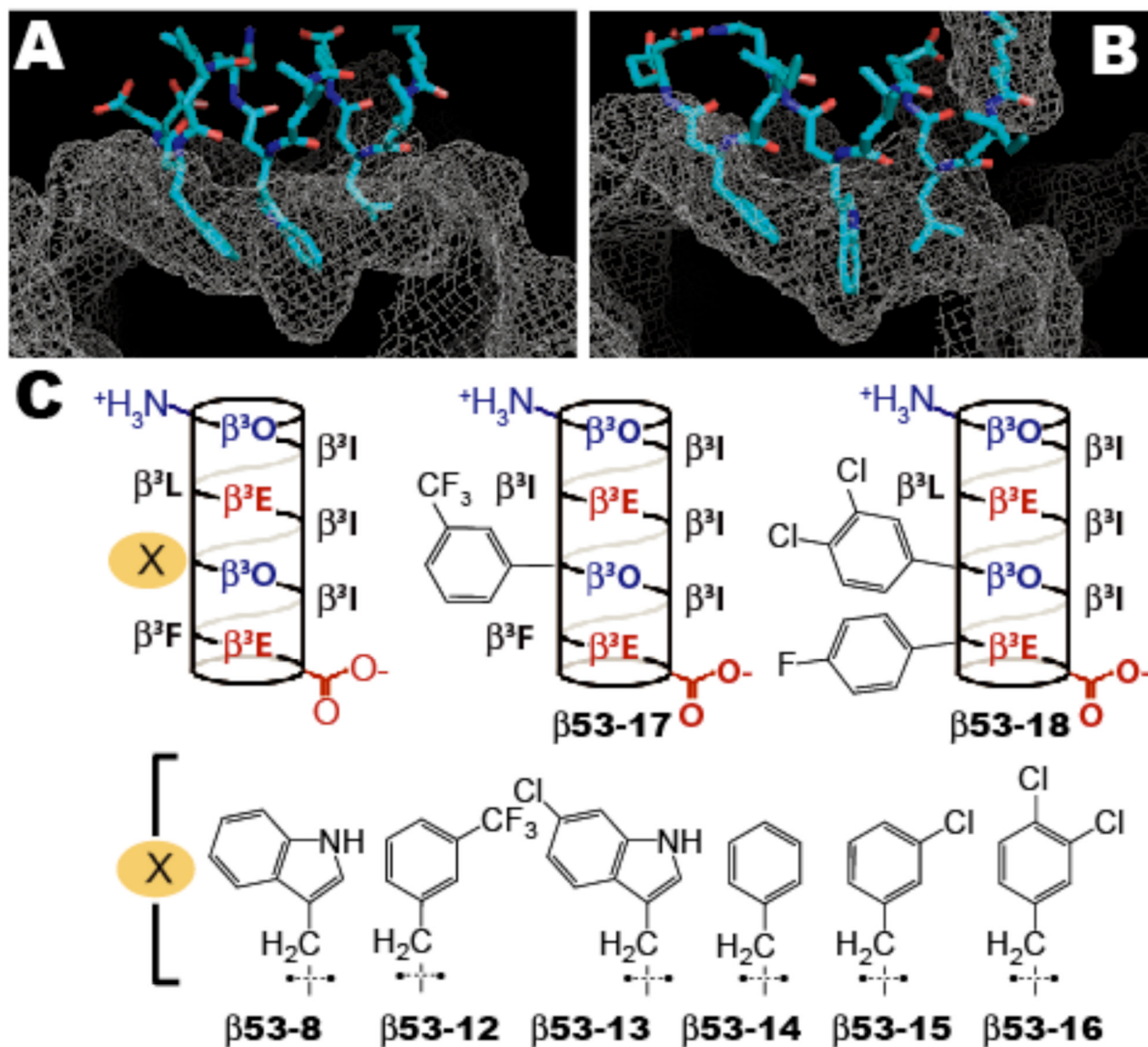
Figure 1. Computationally generated models of β 53 -8 (blue) in complex with (a) hDM2 and (b) hDMX illustrating differences in binding site topologies. (c) Helical net representations of β 3 -peptides studied herein.
