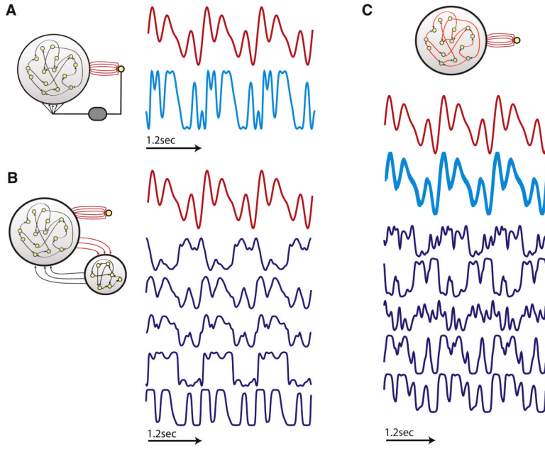
Figure 6. Feedback variants. A) Network trained to produce a periodic output (red trace) when its feedback (cyan trace) is 1.3 \tanh(\sin(\pi z(t - 100 \text{ ms}))) , a delayed and distorted function of the output z(t) (gray oval in circuit diagram). B) FORCE learning with a separate feedback network (circuit diagram). Output is the red trace, and blue traces show activity traces from 5 neurons within the feedback network. C) A network (circuit diagram) in which the internal synapses are trained to produce the output (red). Activities of 5 representative network neurons are in blue. The thick cyan traces are overlays of the component of the input to each of these 5 neurons induced by FORCE learning, \sum_j (J_{ij}(t) - J_{ij}(0)) r_j(t) for i=1K 5 .
