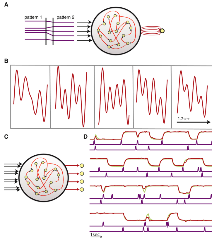
Figure 7. Multiple pattern generation and 4-Bit memory through learning in the generator network. A) Network with control inputs used to produce multiple output patterns (synapses and readout weights that are modifiable in red). B) Five outputs (1 cycle of each periodic function made from 3 sinusoids is shown) generated by a single network and selected by static control inputs. C) A network with 4 outputs and 8 inputs used to produce a 4-bit memory (modifiable synapses and readout weights in red). D) Red traces are the 4 outputs, with green traces showing their target values. Purple traces show the 8 inputs, divided into ON and OFF pairs associated with the output trace above them. The upper input in each pair turns the corresponding output on (sets it to +1). The lower input of each pair turns the output off (sets it to -1). After learning, the network has implemented a 4-bit memory, with each output responding only to its two inputs while ignoring the other inputs.
