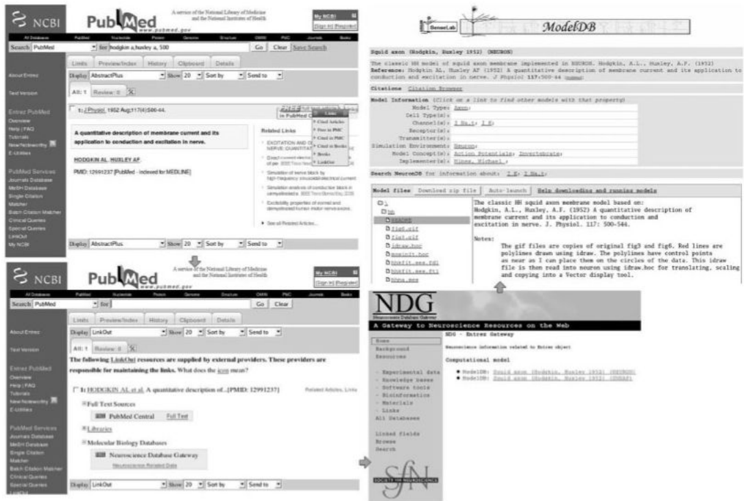
Figure 6. Entrez-LinkOut broker used for ModelDB. When the link to the PUBMED entry in the upper right hand panel is clicked, it opens the page for the original Hodgkin-Huxley computational model in PUBMED shown in the upper left hand panel. The lower left hand panel displays the LinkOut resources in PUBMED for NDG as a link. When that link is clicked, it results in the Hodgkin-Huxley model link in NDG. The lower right panel shows that the Hodgkin-Huxley model is stored in both ModelDB and the SNNAP database housed at University of Texas Medical School in Houston, Texas. Clicking on the link for ModelDB in NDG then results in the original page illustrated in the upper right hand panel.
