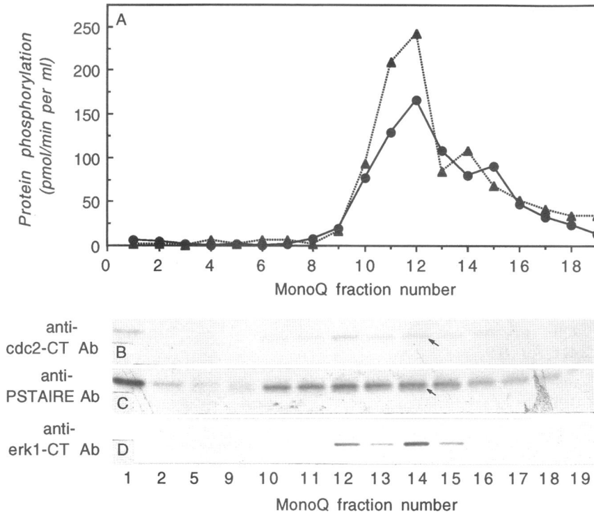
Figure 10. p13 suc1 Binding of nocodazole-stimulated MBP kinase from MonoQ fractions of chick DU249 cells. Two hundred and fifty-microliter aliquots of the MonoQ column fractions shown in Figure 9A were incubated with p13 suc1 -agarose beads for 30 min. The p13 suc1 -agarose beads were suspended and assayed for phosphorylating activity toward 1 mg MBP/ml (●) and 1 mg histone H1/ml (▲) (A). Western blotting was performed with anti-cdc2-CT antibodies (B), anti-PSTAIRE antibodies (C) and anti-erk1-CT antibodies (D). The top and bottom of B and C correspond to the electrophoretic migrations of the prestained marker proteins carbonic anhydrase (33K) and soybean trypsin inhibitor (28K), respectively. The position of p34 cdc2 is indicated with a solid arrow. (D) region of the immunoblots between ~45K and 35K. Similar results were obtained in two separate experiments.
