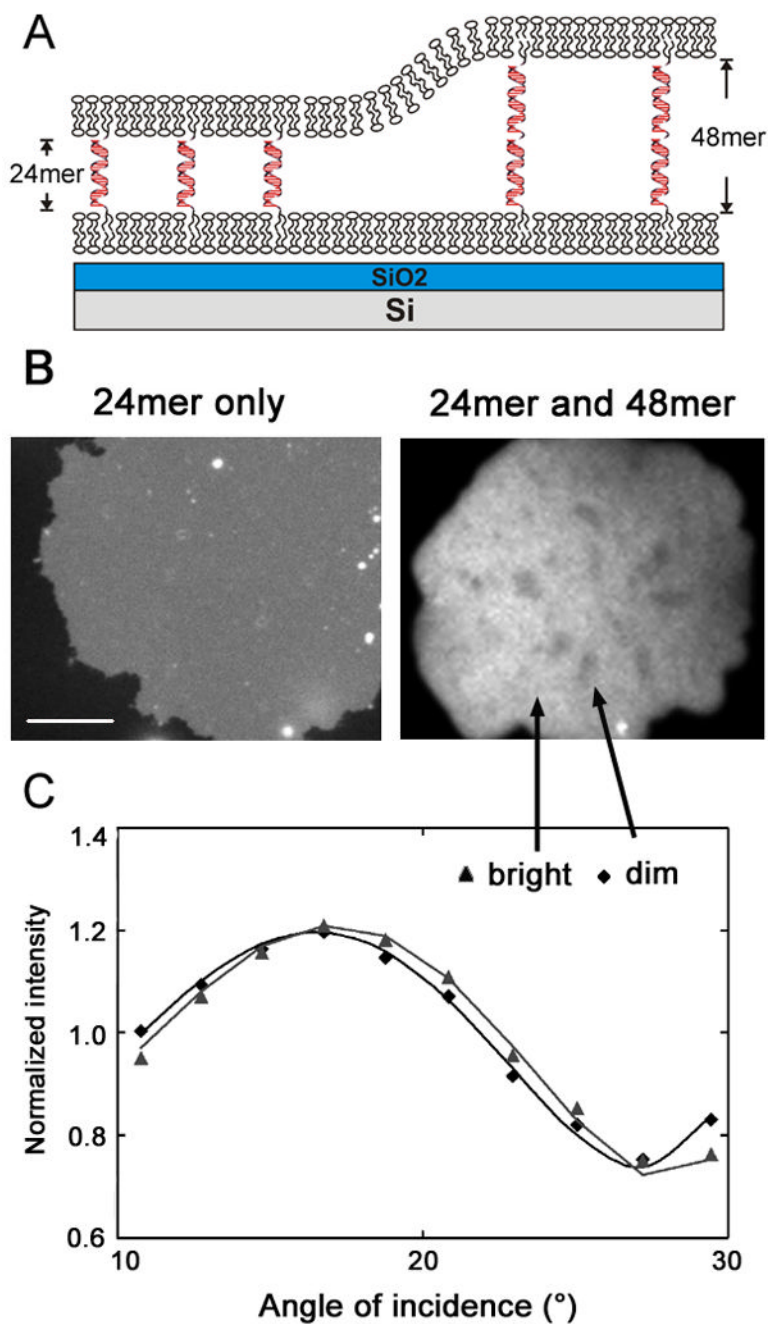
Figure 6. DNA tether segregation by different lengths of DNA hybridization on a mobile SLB (c.f Fig. 1B). (A) Schematic illustration of segregation involving two lengths of DNA hybrids between the mobile membrane surfaces. The substrate is 260 nm of SiO 2 of grown on atomically flat Si to allow for quantitative analysis by VIA-FLIC. (B) Fluorescence image of Texas red labeled tethered bilayer patches. When only 24-mer DNA tethers were used (left, poly A/poly T), the intensity is homogeneous across the membrane. With mixed 24-mer (poly A/poly T) and 48-mer (fully overlapping sequence) tethers, bright and dark domains were observed that indicate regions where the DNA hybrids have segregated by length. Left scale bar is 15 μm, and right image is 10 μm wide. (C) The fluorescence signal as a function of angle of incidence for selected
