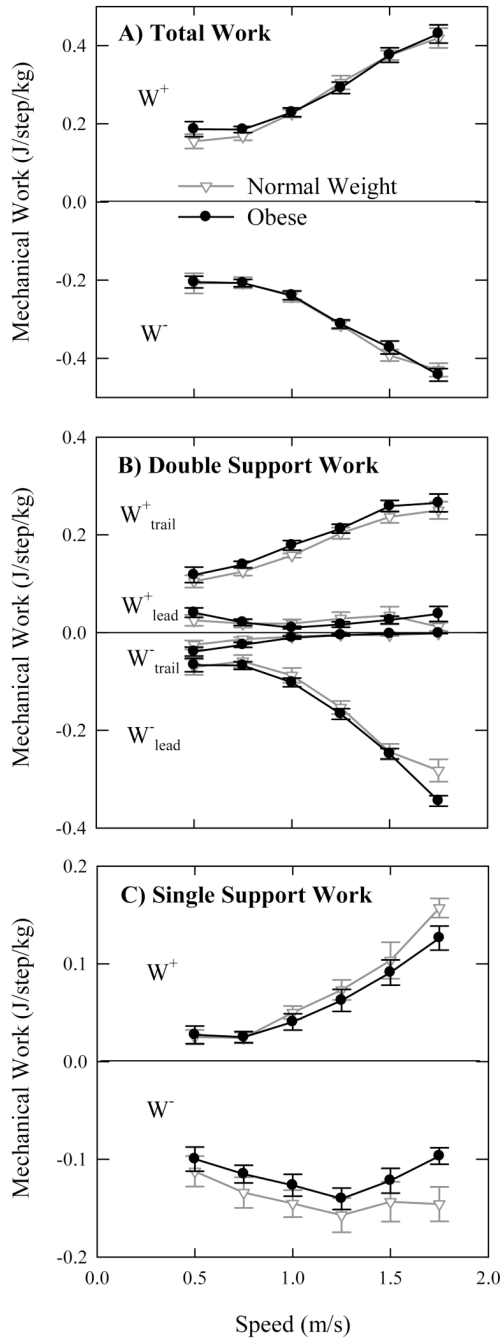
Figure 2. External positive ( W^+ ) and negative ( W^- ) mechanical work (J/step/kg) for normal weight and obese subjects during a step (A), double support (B), and single support (C). All data are mean (SE). There were no significant differences in external work between the groups during a step, double support or single support. During double support, the trailing leg performed primarily positive work while the leading leg performed primarily negative work.
