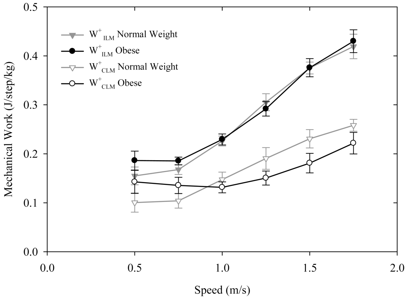
Figure 3. Individual limbs method (ILM) vs. combined limbs method (CLM) measures of total positive external work (J/step/kg) across the range of speeds in obese and normal weight individuals. Data are mean (SE). CLM significantly underestimated positive W_{ext} .
