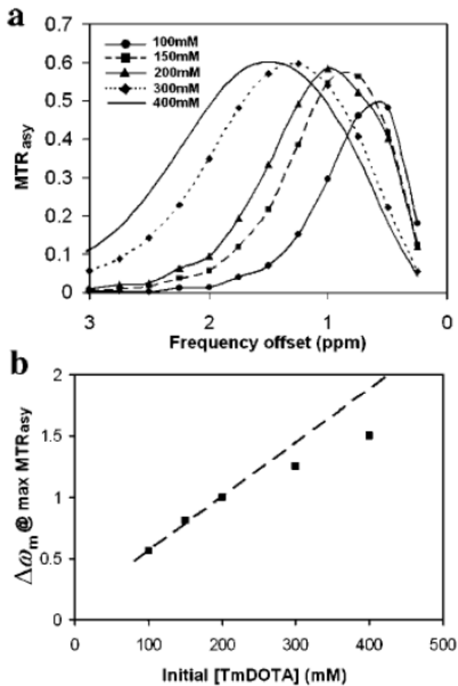
Figure 2. (a) MTR_{asy} versus frequency offset of the presaturation pulse for five liposome samples (diameter \sim 80 nm), each encapsulating a different concentration of TmDOTA from 100 to 400 mM. (b) The frequency offset, \Delta\omega_m , at which MTR_{asy} maximizes as a function of the initial TmDOTA concentration. The dashed line represents a linear fit to the three samples with the lowest initial [TmDOTA].
