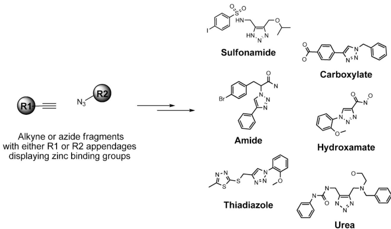
Figure 4. Click chemistry strategy to synthesize selective VIM-2 inhibitors Representative N-substituted and N-unsubstituted 1,2,3-triazoles from alkyne and azide fragments with known or putative zinc binding groups are shown including hydroxamates, amides, ureas, thiadiazoles, carboxylate and sulfonamides.
