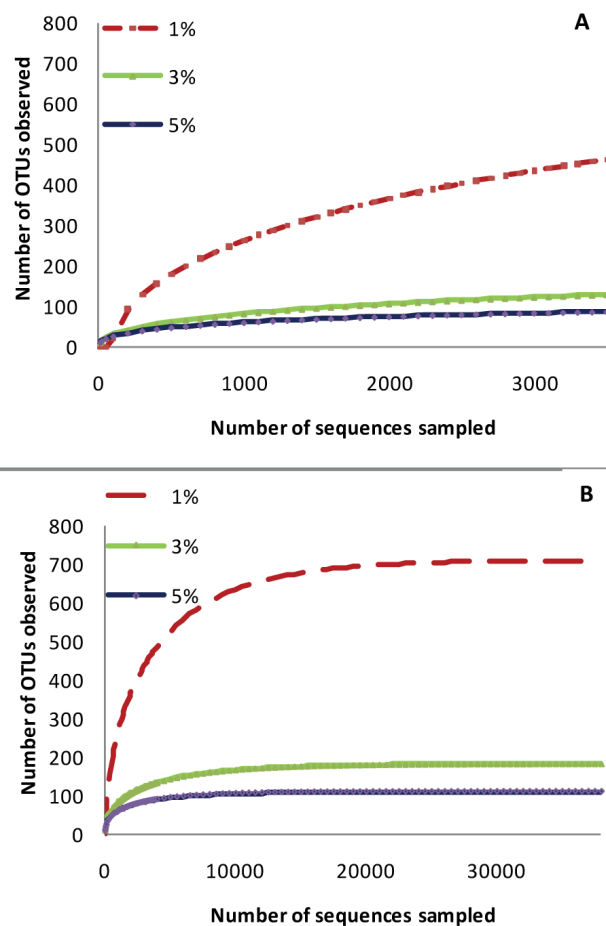
Figure 1 Representative rarefaction curves depicting the effect of 1%, 3%, and 5% dissimilarity on the number of identified and maximum predicted operative taxonomical units (OTUs) in one dog. (A) This plot shows that with the average number of collected sequencing tags per dog (mean \pm SD: 3188 \pm 1091 sequencing tags), we underestimated the number of OTUs at 1% dissimilarity. A reasonable coverage was obtained at 3% and 5% dissimilarity (curves approximate a parallel line to the x-axis). (B) To estimate the maximum number of OTUs at various dissimilarities, a Richards equation was fit to the rarefaction curves. The results indicate that approximately 38,000 sequences would need to be sampled to cover 100% of the expected OTUs in the canine jejunum.
