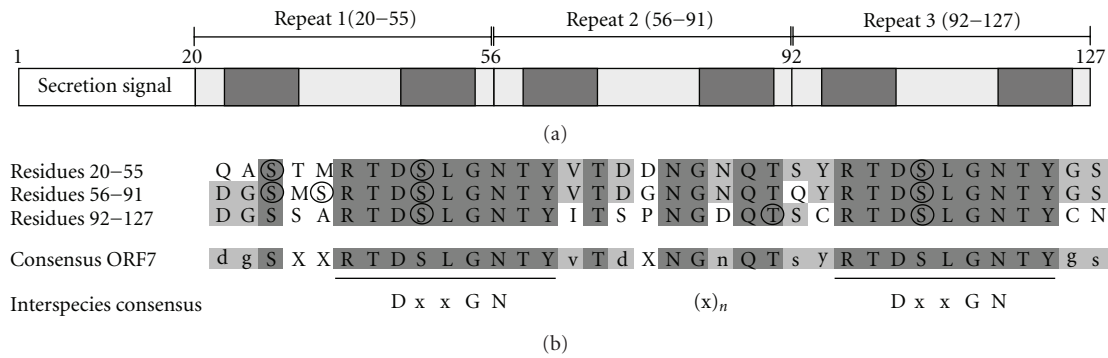
FIGURE 3: ORF7 of plasmid pYe4449-2 encodes a putative new repeat protein with a high content of phosphorylatable amino acids. (a) Scheme of the arrangement of the ORF7-encoded hypothetical protein. The nonameric repeat module “RTDSLGN TY” occurring twice in each repeat is indicated by dark grey boxes. (b) Alignment of the protein repeat segments encoded by ORF7, residues identical in all three repeats are highlighted against a dark grey background and residues identical in two of the three repeats are highlighted against a light grey background. The repeat module “RTDSLGN TY” occurring twice in each repeat is indicated by a bar below the consensus sequence. Below these bars, the interspecies repeat motif “DxxGN(x) n DxxGN” is given as deduced from the closest homologues of ORF 7 (BACOVA_04330; NE2449; MPG2080.02246). Serine and threonine residues most likely to be phosphorylated in a eukaryotic background according to NetPhos 2.0, server predictions (score 0.968 and above) were indicated by circles.
