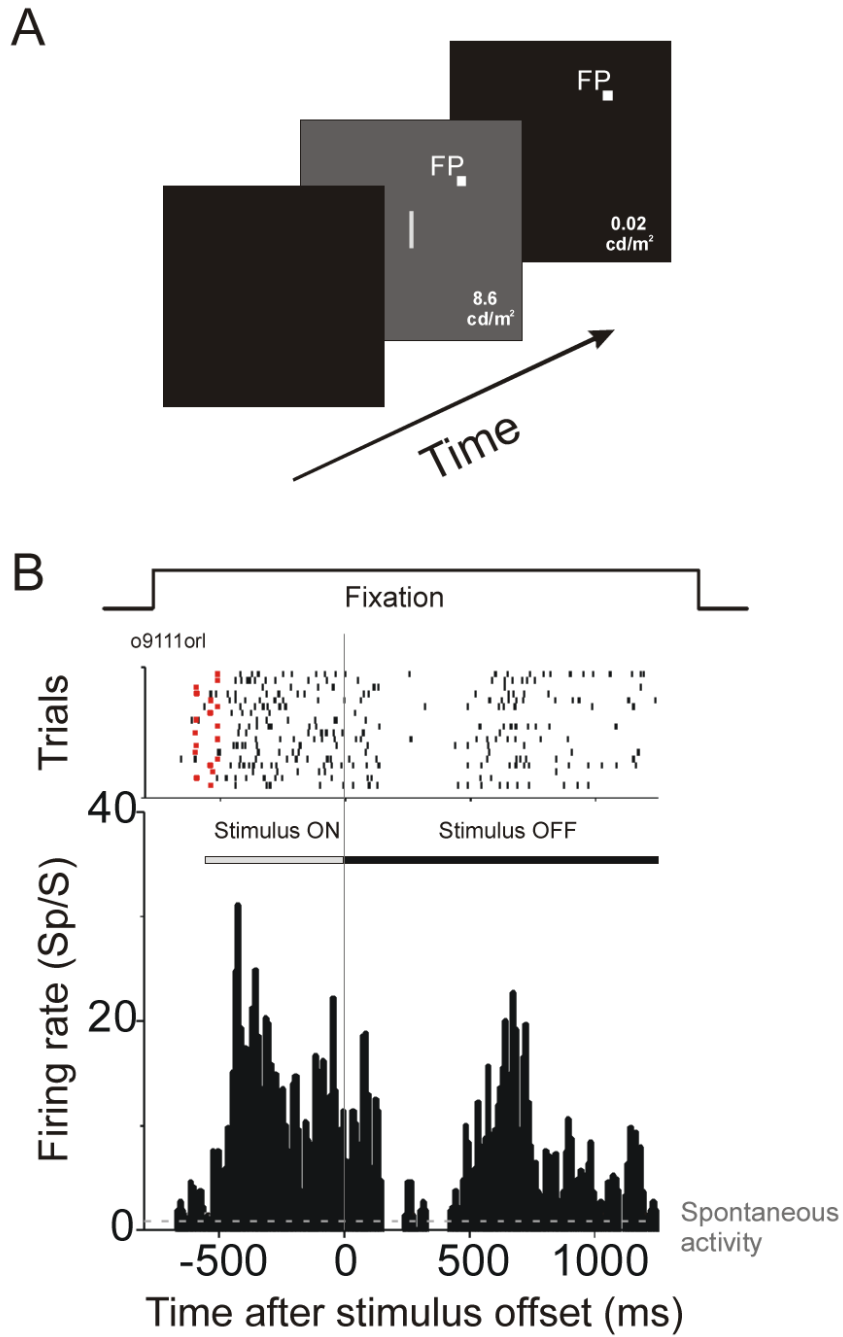
Figure 1. Overview of the physiological experiment. A. The visual stimulus was a bar of light presented on a uniform gray background. The bar was turned off simultaneously with a change from gray to black background. B. Raster plot and PSTH from a representative V1 neuron. The top of this panel shows the animal’s fixation period. In the raster plot below, each short bar represents a spike. Spikes are aligned relative to stimulus offset (time zero). The small red square at the beginning of each trial indicates the stimulus onset time. The raster plot and PSTH show that after stimulus offset, this neuron gave a transient off response lasting for about 150 ms, followed by a period with low activity and then a strong activity rebound starting around 450 ms and lasting for about 600 ms.
