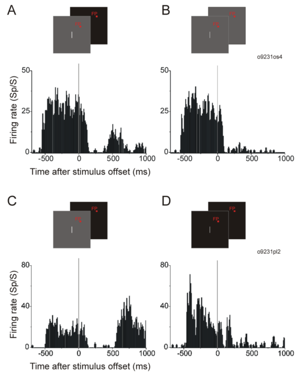
Figure 6. Importance of background offset in rebound activity. A. and C. show for 2 neurons that when the stimulus bar was switched off simultaneously with the background, clear rebound activity was observed. B. When the stimulus bar was turned off but the background remained gray, rebound activity was much weaker or absent (same neuron as A ). D. When the background was static black, the visual response was stronger than with the gray background ( C ), but there was little, if any, rebound activity around 500 ms after stimulus offset (same neuron as C ).
