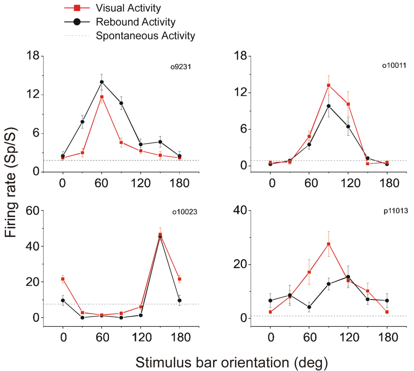
Figure 3. Effect of stimulus orientation on visual response and rebound activity. Red curves show orientation tuning functions for four V1 neurons based on the visual response 0 - 500 ms after stimulus onset. Black curves show the dependence of rebound activity (500-1000 ms after stimulus offset) on stimulus orientation. Error bars show standard errors.
