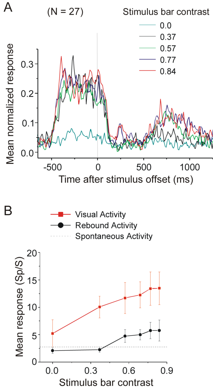
Figure 2. Effect of stimulus contrast on neural activity. A. Averaged normalized PSTHs of 27 neurons in response to a stimulus bar with different luminance contrasts. The magnitude and duration of the rebound activity increased as contrast increased. At contrast levels of 0.77 and 0.84, an additional early activity peak was found about 200 ms after stimulus offset. Responses are aligned at stimulus offset. B. Mean visual responses calculated 0 to 500 ms after stimulus onset (red symbols) and mean rebound activity calculated 500 to 1000 ms after stimulus offset (black symbols). Both visual responses and rebound activity increased with contrast. Mean spontaneous activity across the 27 neurons is indicated by the dashed line.
