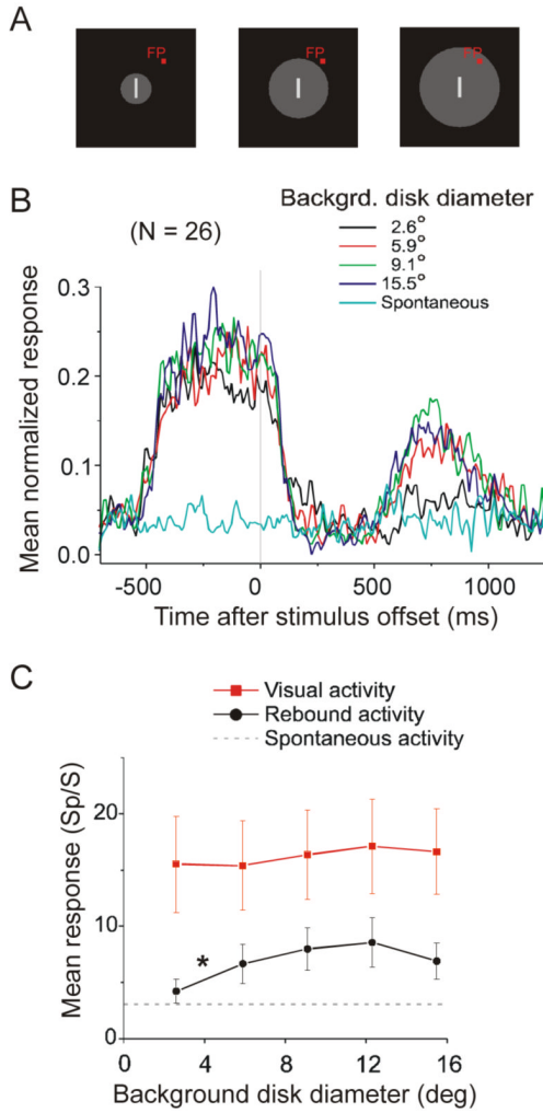
Figure 5. Rebound activity depends on background size. A. The gray background varied in size from 2.6° to 15.5°. B. Averaged normalized PSTHs of 26 neurons as background size varied. To avoid excessive clutter, responses to only 4 of the 5 background sizes are shown. C. The mean firing rates of the visual responses were calculated 0 to 500 ms after stimulus onset (red symbols) and the mean rebound activities were calculated 500 to 1000 ms after stimulus offset (black symbols). With a diameter of 2.6°, rebound activity was significantly weaker than with larger disk diameters (indicated by the asterisk, see text), but visual responses did not differ. Mean spontaneous activity across the 26 neurons is indicated by the dash line.
