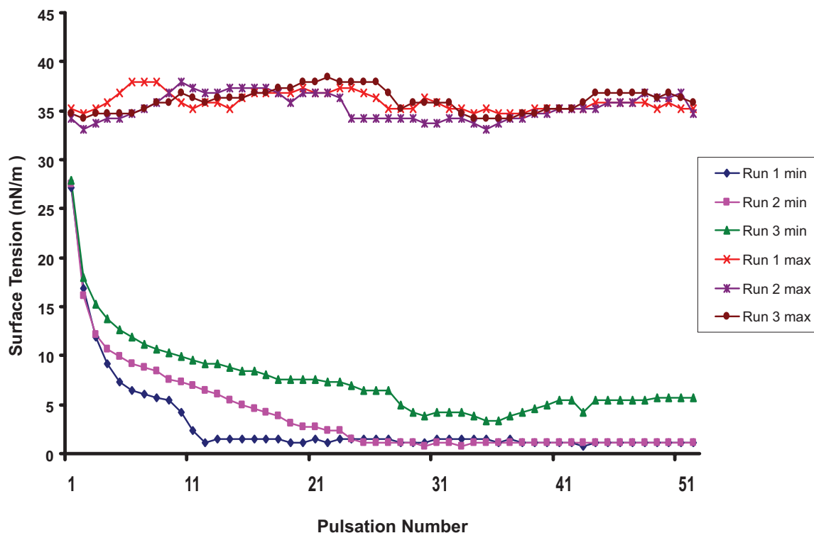
Figure 1 Surface tension properties of surfactant (BLES ® ). Maximum (max) and minimum (min) surface tension (nN/m) as determined by pulsating bubble meter in three runs as the bubble formed at the surface of the air/surfactant interface is subject to 20 pulsations per minute for 2 ½ minutes. After 25 pulsations the surface tension reaches a minimum of 2 \pm 2 nN/m.
