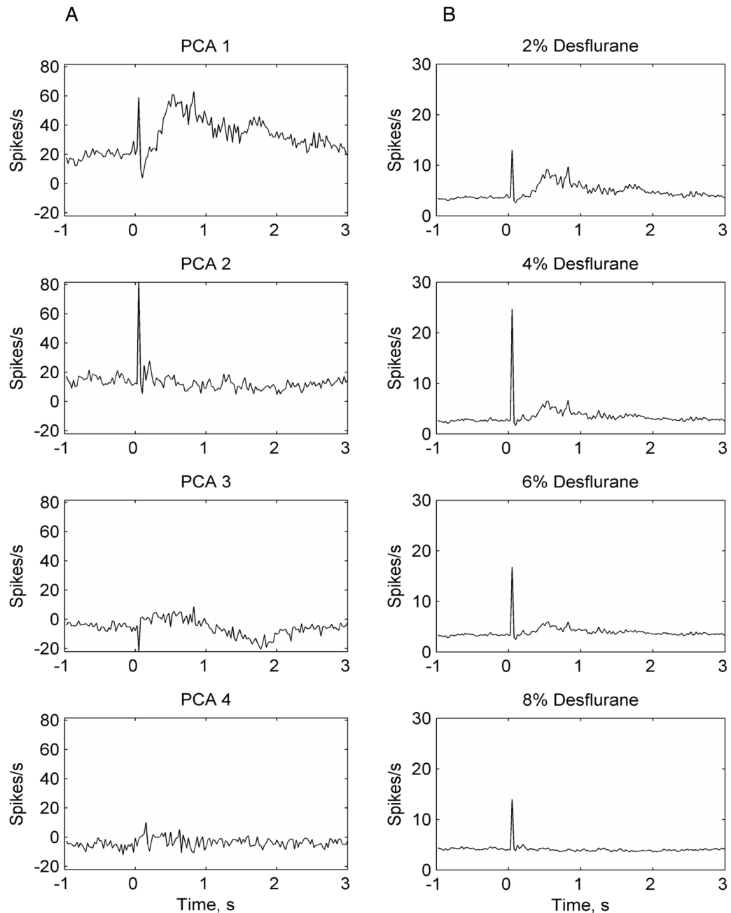
Figure 6. Illustration of modeling the population response to flash using Principal Components Analysis and the General Linear Model in one experiment. Panel A shows the first four predicted peristimulus spike rate histograms (component scores) from the corresponding four principal components. Panel B shows spike rate responses at various anesthetic concentrations as modeled by the first two canonicals on Panel A. Although three principal components were significant, the first two components captured the responses of interest. Note the early + late response represented in the first principal component (PCA 1) and the early only response represented in the second principal component (PCA 2). A concentration-dependent
