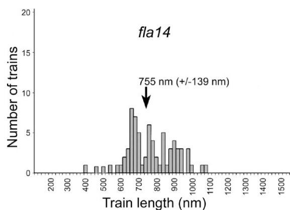
Figure 3. Length distribution of IFT trains in WT and fla14 flagella. (a) Table of the number of clearly identifiable and measurable long and short IFT trains in WT and fla14 flagella. (b and c) Histograms of the length distributions of IFT trains in flagella of WT (b) and fla14 (c) cells. The arrows mark the mean length ( \pm SD) of the long (grey) and short (black) IFT trains.
