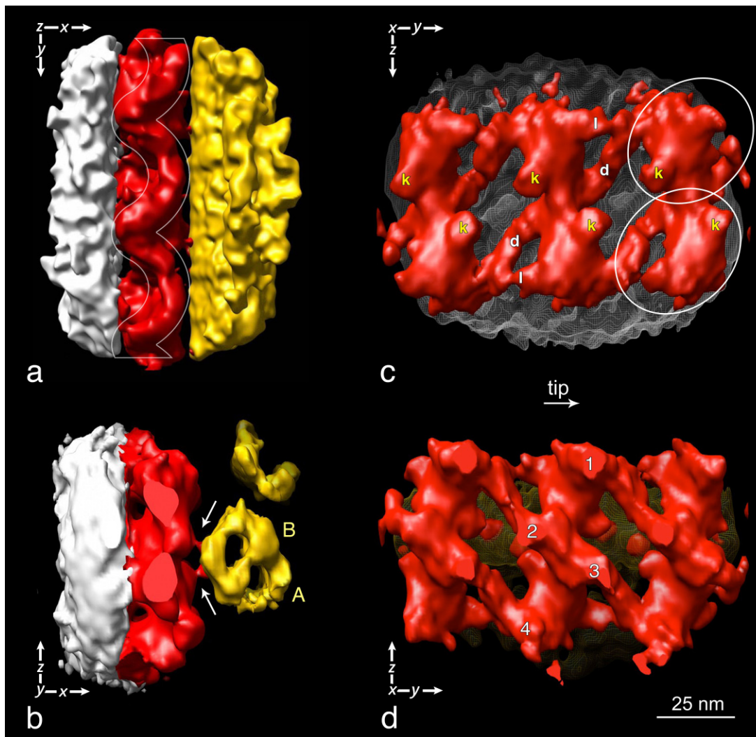
Figure 7. Four different views of a surface-rendering representation of the 3D model of IFT particles in fla14 flagella. Colors have been assigned to sub-volumes of the density map corresponding to different flagellar structures using the same color coding shown in Figs. 5 and 6 (white, flagellar membrane; red, IFT particles; yellow, MT doublets). In this and subsequent figures, the images are oriented so the flagella point down or to the right. (a) The white lines highlight the festooned profile of the IFT particles. The same wave pattern is seen in Fig. 6, panel 1, and Fig. 2 (f–o). (b) Cross-section view of the same model oriented so that the tip of flagellum points toward the reader. The white arrows indicate the position of the links between each IFT particle and the B subunit of the MT doublet (B). A, A subunit of the MT doublet. (c) Three pairs of IFT particles lying on the flagellar membrane (white wire net pattern) as seen from the interior of the axoneme. Oblique links (d) connect neighboring particles (white ovals) along each strand. Links (l), oriented parallel to the longitudinal axis of IFT trains, connect the heads of adjacent particles. The position of the links between IFT particles and the B subunit of the MT doublet are labeled with a k, and may be the kinesin-2 motors. (d) The pairs of IFT particles as seen from the exterior of the flagellum. The yellow net behind them represents the outer surface of an MT doublet. 1, 2, 3, and 4 indicate the contact points between IFT particles and the flagellar membrane. Video 2 shows a rotation of the surface-rendered model.
