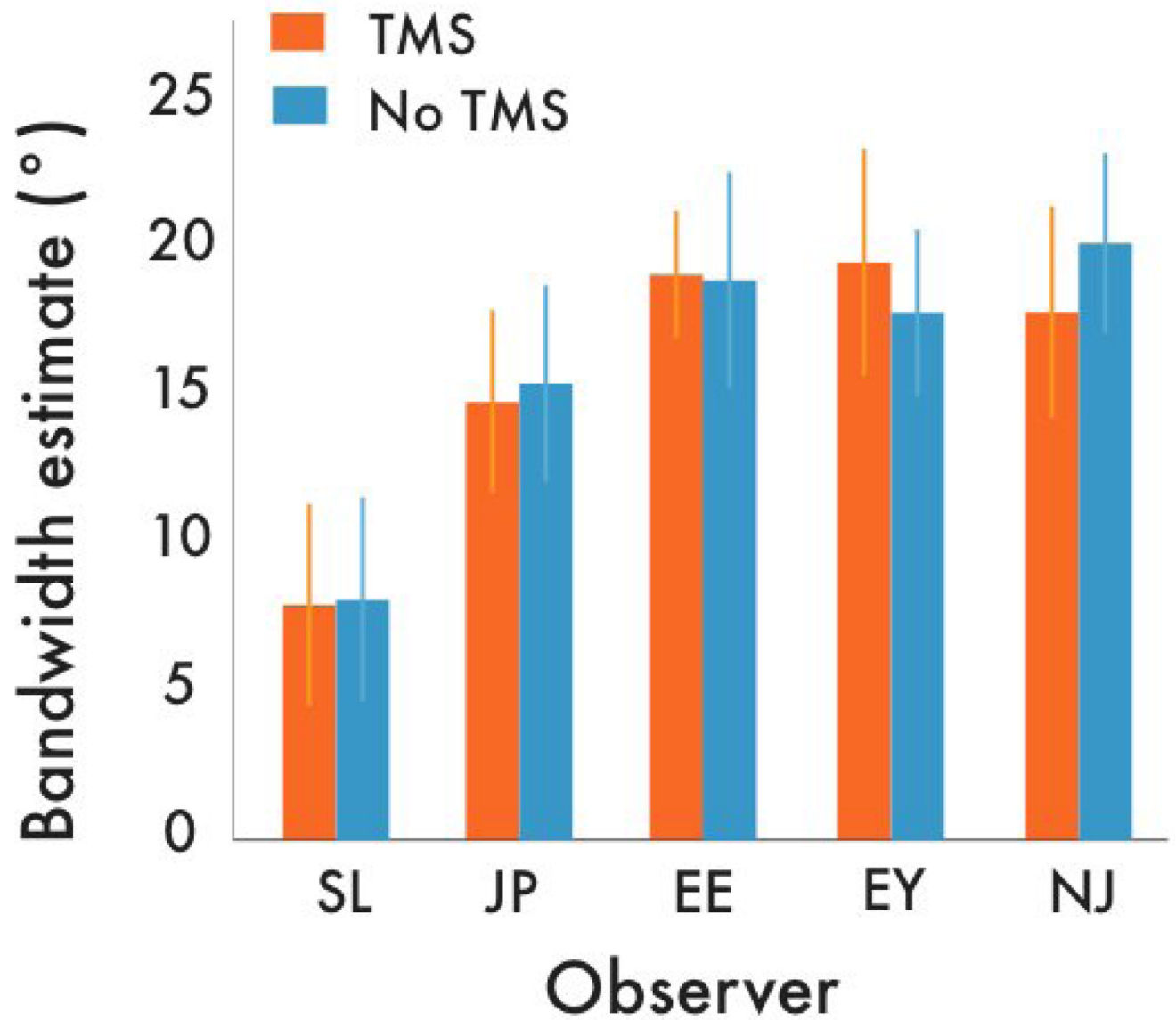
Figure 2. Orientation tuning bandwidth estimates measured inside and outside of the rTMS site. Although intracortical activity was depressed by TMS, there was no significant change in the bandwidth of orientation selectivity. Error bars correspond to the bootstrapped 95% confidence intervals.
