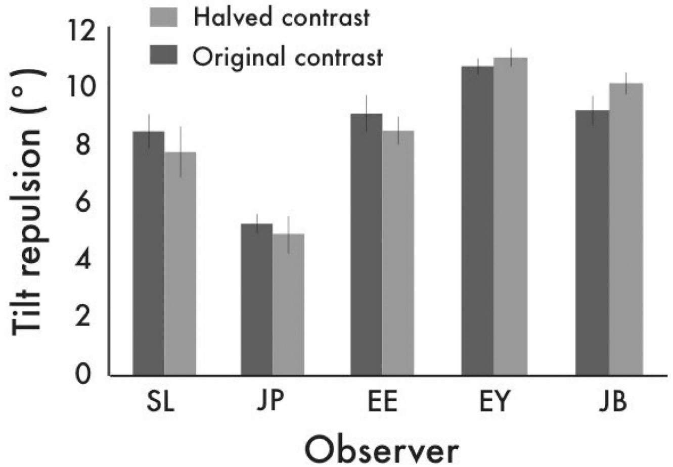
Figure 4. Halving the contrast of the inducer and test stimuli did not significantly affect the magnitude of the tilt repulsion illusion. Error bars correspond to \pm 1 s.e.
