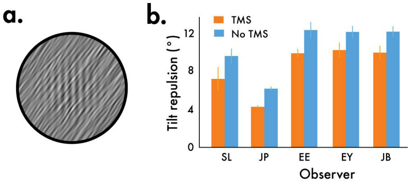
Figure 3. TMS diminishes the tilt repulsion illusion. (a) A demonstration of the tilt repulsion illusion. Although the physical orientation of the grating is vertical, when embedded within oriented noise, the grating appears to be tilted away from the noise orientation. This illusion is commonly attributed to lateral interactions in early visual cortex. (b) When the stimulus was presented outside the TMS site (blue bars), observers perceived the grating to be tilted away from vertical. However, under TMS, the magnitude of this illusion weakened.
