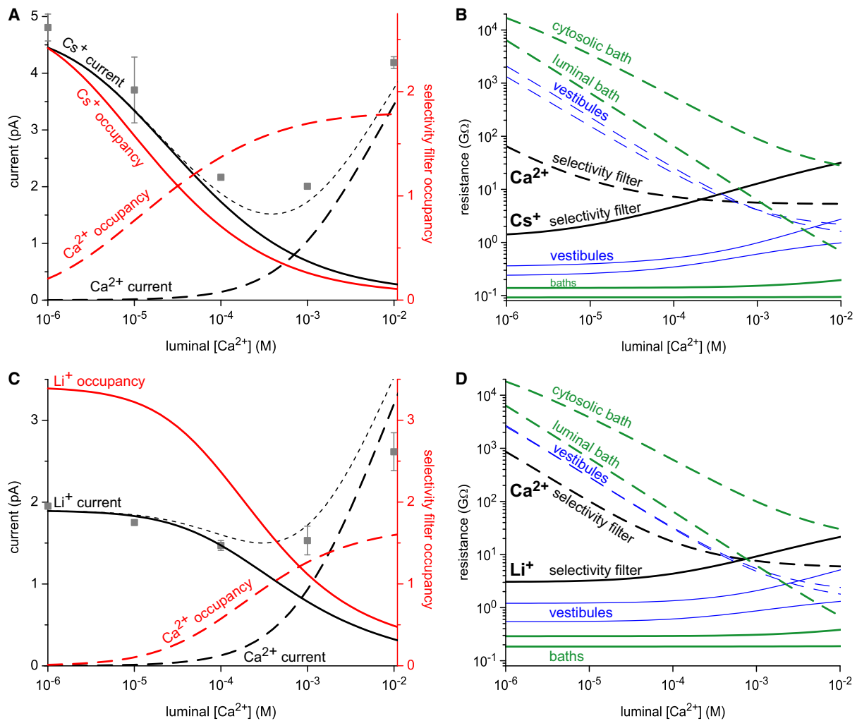
FIGURE 3 (A) \text{Ca}^{2+} and \text{Cs}^{+} current (black lines, left axis) and number of \text{Ca}^{2+} and \text{Cs}^{+} in the selectivity filter (red lines, right axis) as [\text{Ca}^{2+}]_{\text{lum}} is increased. The net current is shown with the dotted line and the experimental results are shown with gray squares. (B) The resistances of \text{Cs}^{+} (solid lines) and \text{Ca}^{2+} (dashed lines) in the selectivity filter (black lines), the cytosolic and luminal vestibules (blue lines), and the baths (green lines). (C and D) Same as panels A and B with \text{Li}^{+} substituted for \text{Cs}^{+} . The applied voltage is 10 mV.
