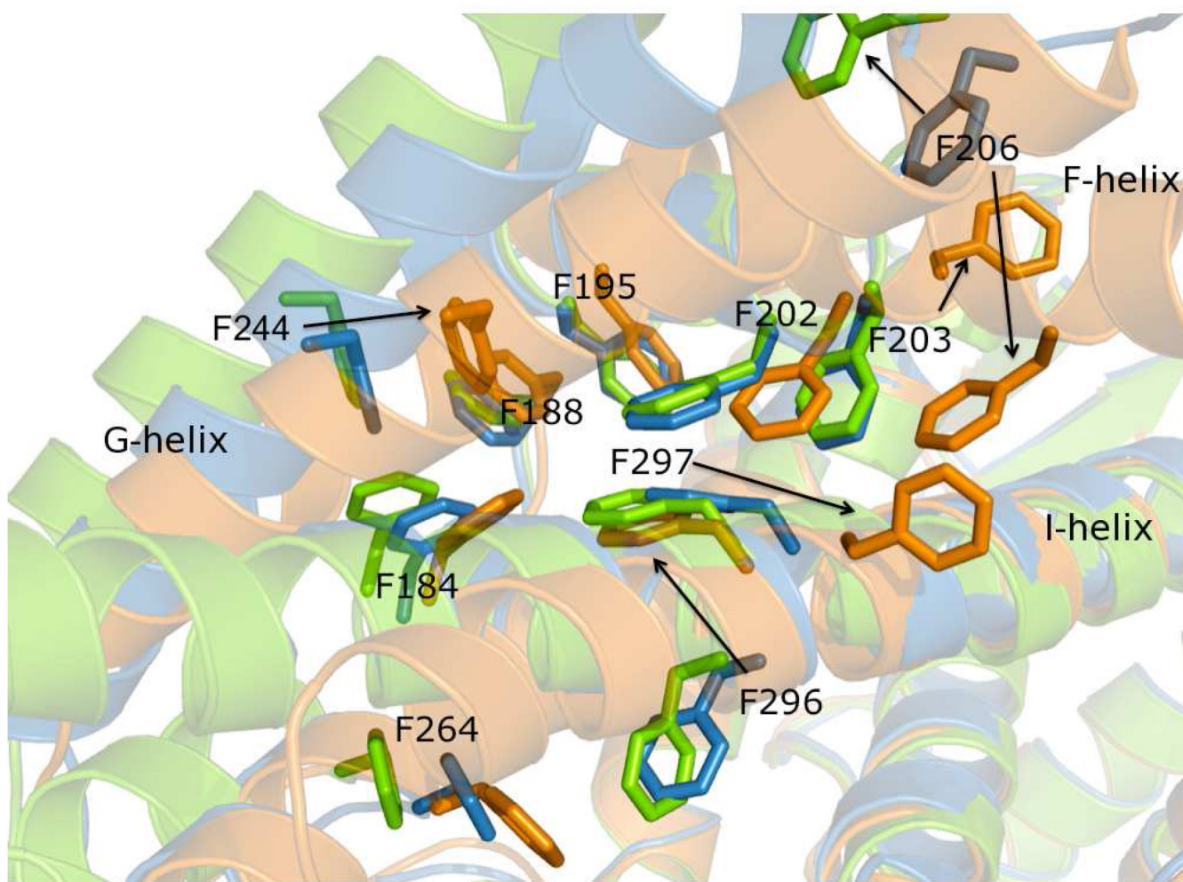
Figure 7. Transparent ribbon and stick diagram of CYP2B4 overlays highlighting the Phe cluster at the F-, G-, and I-helix intersection. The 4-CPI, 1-PBI, and bifonazole structures are shown in orange, blue, and green respectively. The cluster of Phe residues at this helical intersection reposition their side chains in each structure to fill void volumes as the F-G helix cassette pivots across the I-helix. Black arrows indicate large shifts in Phe location. The largest changes come at residue numbers 203, 206, 244, 296, and 297. The position of Phe 203 is conserved in the 1-PBI and bifonazole structures, but this residue swings around to the other side of the F-helix in the 4-CPI structure. Phe 206 diverges significantly in all structures based on the unraveling of the F-helix. The 4-CPI Phe 296 occupies the same place as Phe 297 in the 1-PBI and bifonazole structures. Phe 297 of the 4-CPI structure rotates around to interior of the active site.
