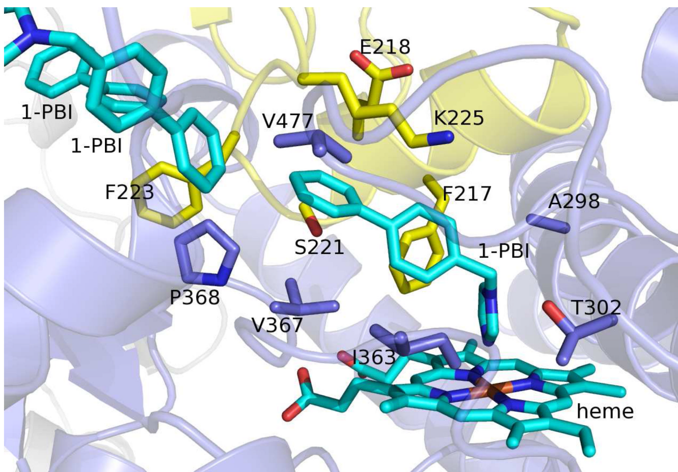
Figure 5. Semi-transparent ribbon and stick diagram of the CYP2B4:1-PBI complex active site. Chain A is colored blue and chain B is colored yellow. Heme and 1-PBI molecules are shown as cyan sticks. Side chains of residues identified within a 5 Å radius of the 1-PBI coordinated to the heme iron are shown as blue and yellow sticks.
