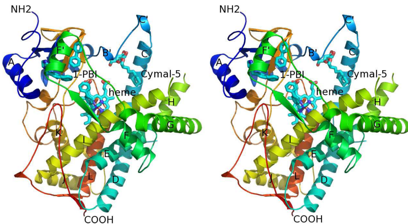
Figure 3. Divergent stereoview of CYP2B4:1-PBI complex monomer A chain ribbon diagram. The chain is colored from blue to red from the N-terminus to the C-terminus respectively. Heme, 1-PBI, and Cymal-5 molecules are shown as cyan sticks. The F-, F'-, and G-helices rest across the I-helix forming a lid over the active site.
