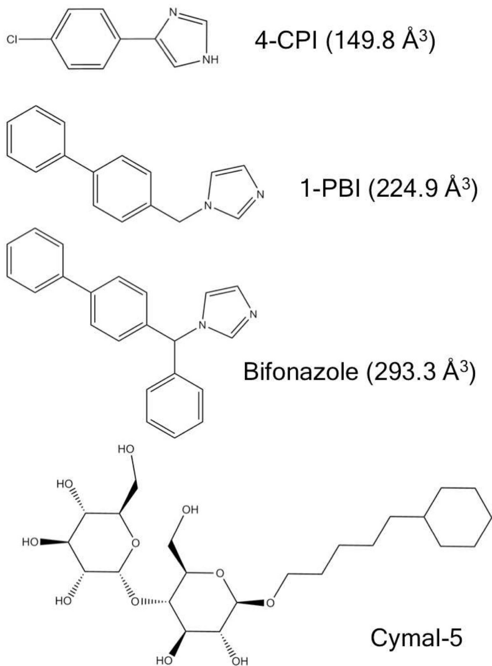
Figure 1. Stick model structures of 1-PBI, 4-CPI, and bifonazole inhibitor molecules and Cymal-5 detergent. Volumes for inhibitors calculated using http://www.molinspiration.com/cgi-bin/ properties are listed in parantheses.
