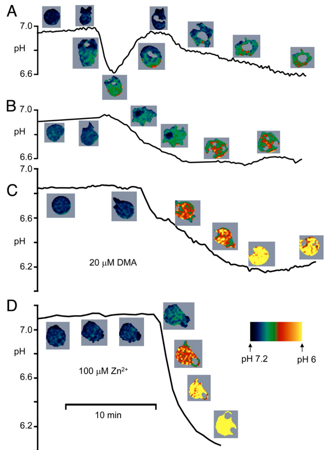
Fig. 2. Time course of pH_i changes in 4 phagocytosing neutrophils. Pseudocolor images of each cell are positioned near the corresponding time point. The spatially averaged pH_i of the cell is plotted, including only areas of cytoplasm above a threshold level of fluorescence intensity; areas below the cutoff (e.g., in phagosomes) are blanked. Acidification invariably occurred rapidly after productive contact with OPZ, often followed by rapid recovery (A), but sometimes not (B). In cells pretreated with 20 \mu M DMA to inhibit Na^+/H^+ antiport (C), or 100 \mu M Zn^{2+} to inhibit proton current (D), pH_i decreased farther and did not recover.
