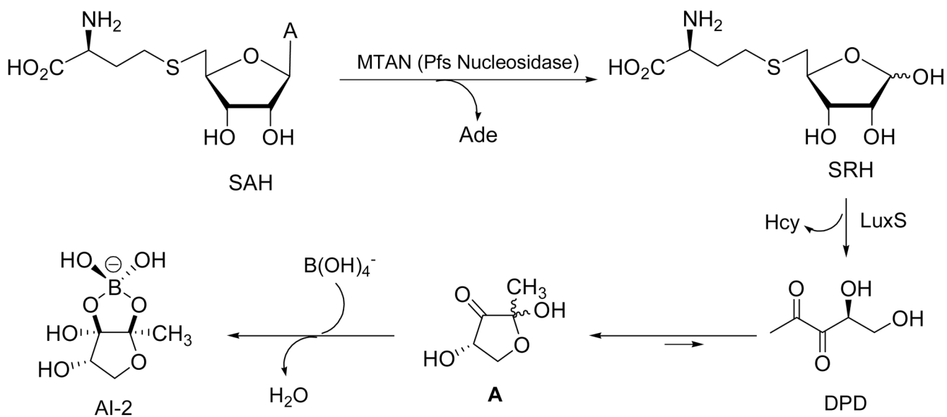
Figure 1. Enzymatic conversion of SAH by MTAN and LuxS: Biosynthetic pathway to AI-2.
