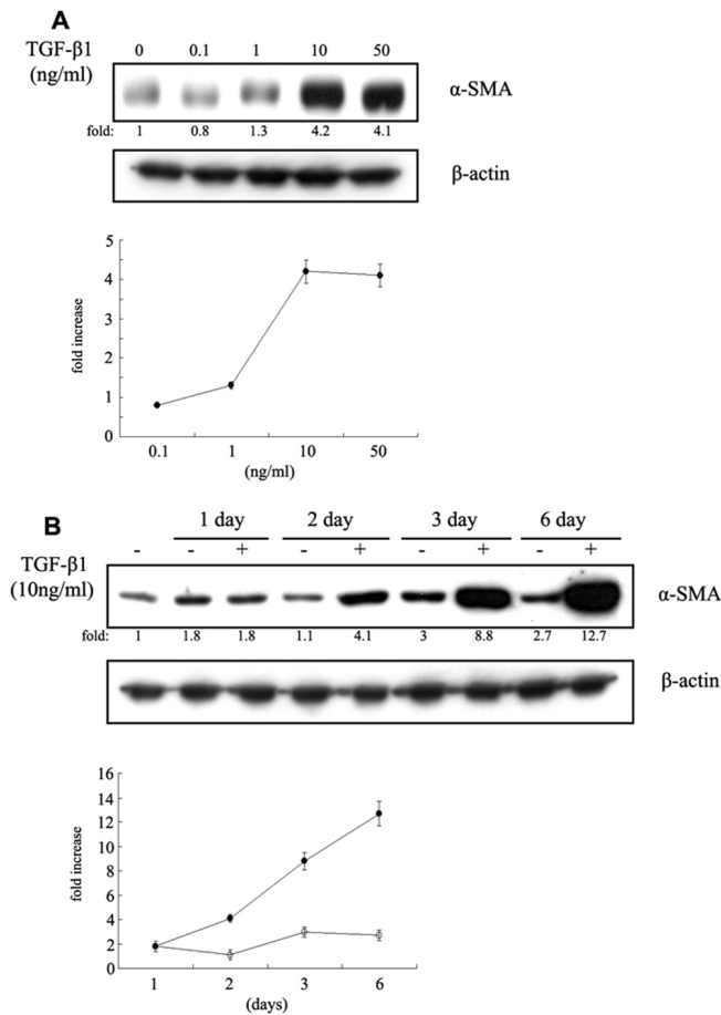
Figure 1. Representative western blot bands for α-smooth muscle actin. A: Dose-response effects: fibroblasts were exposed to various concentrations of transforming growth factor (TGF)-β1 for 72 h. B: Time-response effects: fibroblasts were incubated with or without 10 ng/ml of TGF-β1 for up to 6 days. β-actin was used as an internal control. Densitometric data represent the mean±SD of results from three independent experiments.
