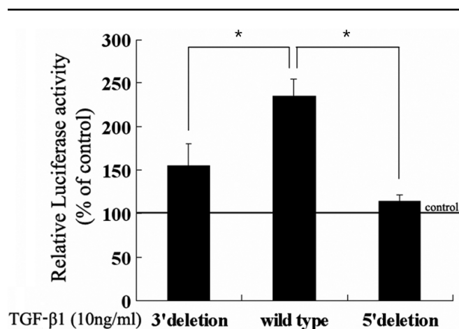
Figure 5. Promoter deletion assay for interleukin-6 ( IL-6 ). Three recombinant plasmids, in which different fragments of the activator protein-1 (AP-1)-binding site on the human IL-6 promoter were deleted, were used. After transfection with each plasmid, fibroblasts were incubated with 10 ng/ml transforming growth factor (TGF)- \beta 1 for 72 h. The luciferase activity was then determined and expressed as the percent of the no-TGF- \beta 1 treatment control. Data represent the mean \pm SD of results from three independent experiments. The asterisks refer to a significant difference ( p < 0.001 ) compared to the wild type.
