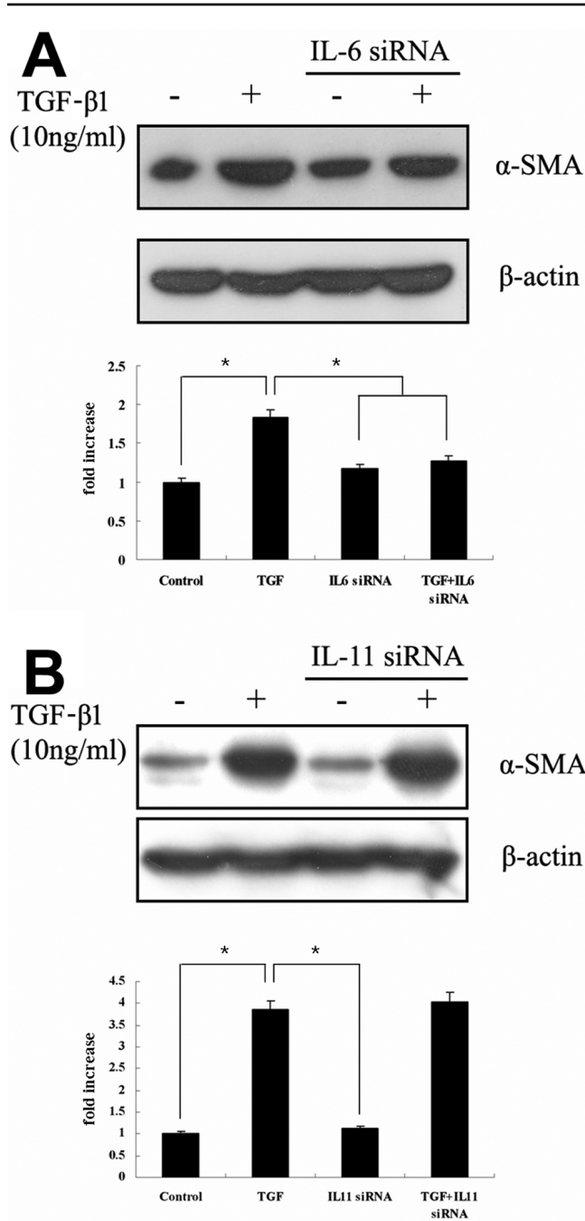
Figure 3. RNA interference assay for IL-6 and IL-11 . After administering small interfering RNAs targeting IL-6 (A) and IL-11 (B), fibroblasts were exposed to 10 ng/ml transforming growth factor (TGF)- \beta 1 for 72 h. Then, the expression of \alpha -smooth muscle actin ( \alpha -SMA) was evaluated using western blots. Densitometric data represent the mean \pm SD of results from three independent experiments. The asterisks refer to a significant difference compared to TGF- \beta treatment only ( p < 0.001 ).
