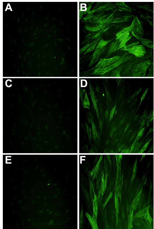
Figure 4. Immunofluorescent analysis of the expression of \alpha -smooth muscle actin. A: No treatment control, B: 10 ng/ml transforming growth factor (TGF)- \beta 1 for 72 h, C: IL-6 -specific small interfering (si)RNA, D: IL-6 -specific siRNA plus 10 ng/ml TGF- \beta 1 for 72 h, E: IL-11 -specific siRNA, and F: IL-11 -specific siRNA plus 10 ng/ml TGF- \beta 1 for 72 h. The secondary antibody was conjugated with fluorescein isothiocyanate, resulting in green fluorescence. Total magnification was 400 \times .
