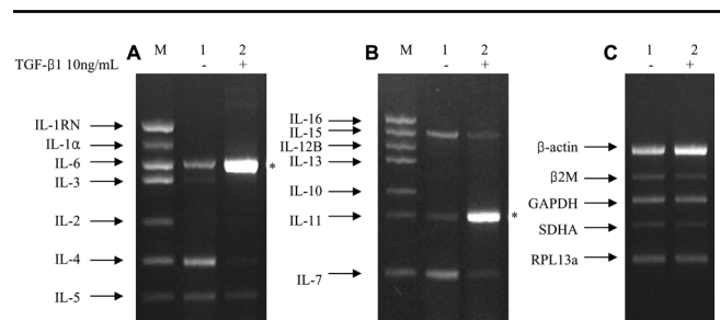
Figure 2. Multiplex reverse transcription PCR. Multiplex reverse transcription PCR sets for interleukins (ILs; A , B ) and housekeeping genes ( C ). For each set of data, lane 1 represents the control group with no transforming growth factor (TGF)-β1 treatment and lane 2 represents the study group with 10 ng/ml TGF-β1 treatment for 72 h. Lane M contains positive markers. GAPDH , glyceraldehyde-3-phosphate dehydrogenase; IL-1RN , interleukin-1 receptor antagonist; RPL13a ; SDHA , succinate dehydrogenase complex subunit A; β2M , β2-microglobulin. Two asterisks refer to a significant increase ( p < 0.001 ) in expression of IL-6 and IL-11 in the presence of TGF-β1.
