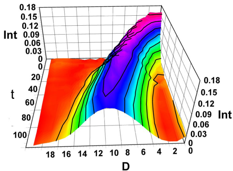
Figure 3. 3D plot of the evolution of D-distribution as a function of time for 2 h following mixing in n -propanol-OD. Removing the native C-13 isotope distribution from the data at all the time points reveals an envelope that represents the deuterium distribution. Int is signal intensity, D is the number of deuteria taken up by the dimer, and t is the time of exchange in min.
