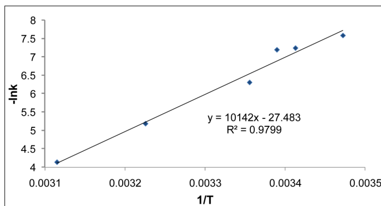
Figure 6. Temperature dependence of the rate constant for the dimer dissociation of gramicidin in n -propanol-OD. The points are the experimental data, and the line is the linear-regression fit obtained using Microsoft Excel.
