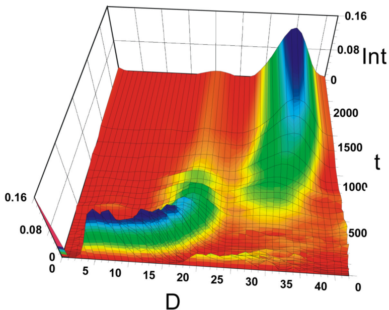
Figure 4. Three-dimensional view of the time-dependent evolution of the D-distribution for HDX of (GA_2 + 3Na)^{3+} in n -propanol-OD. The plot shows the evolution of a second-species at long times. Int is signal intensity, D is the number of deuteria taken up by the dimer, and t of exchange is time in minutes. The low intensity distributions at approximately 20 D's at t = 0 may represent an impurity.
