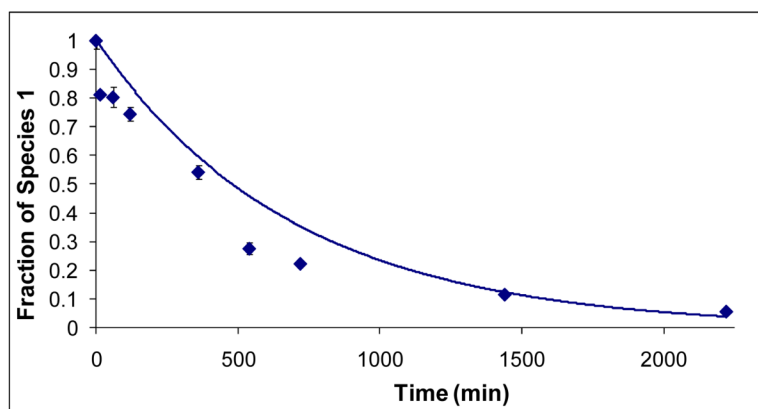
Figure 5. Disappearance of the partially protected species, representing unfolding of the dimer. The points are the experimental data, and the curve is the first order kinetic fit to the data.
