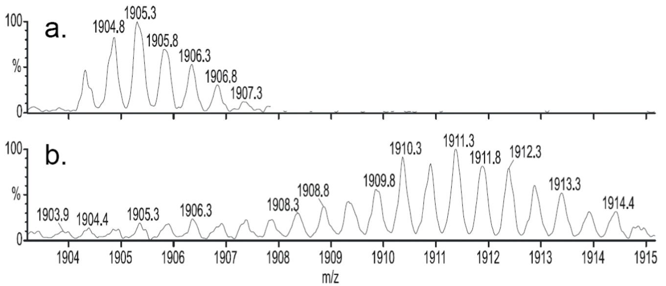
Figure 2. (M_2 + 2Na)^{2+} region of gramicidin A exchanging in propanol before (a.) and after (b.) 1 h of mixing in n -propanol-OD. The data show the uptake of ~ 12 D's out of a possible 42 in the dimer.
