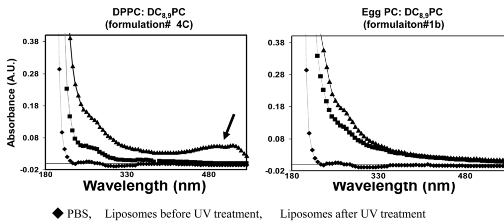
Figure 4. Spectral Properties of UV-treated liposomes
