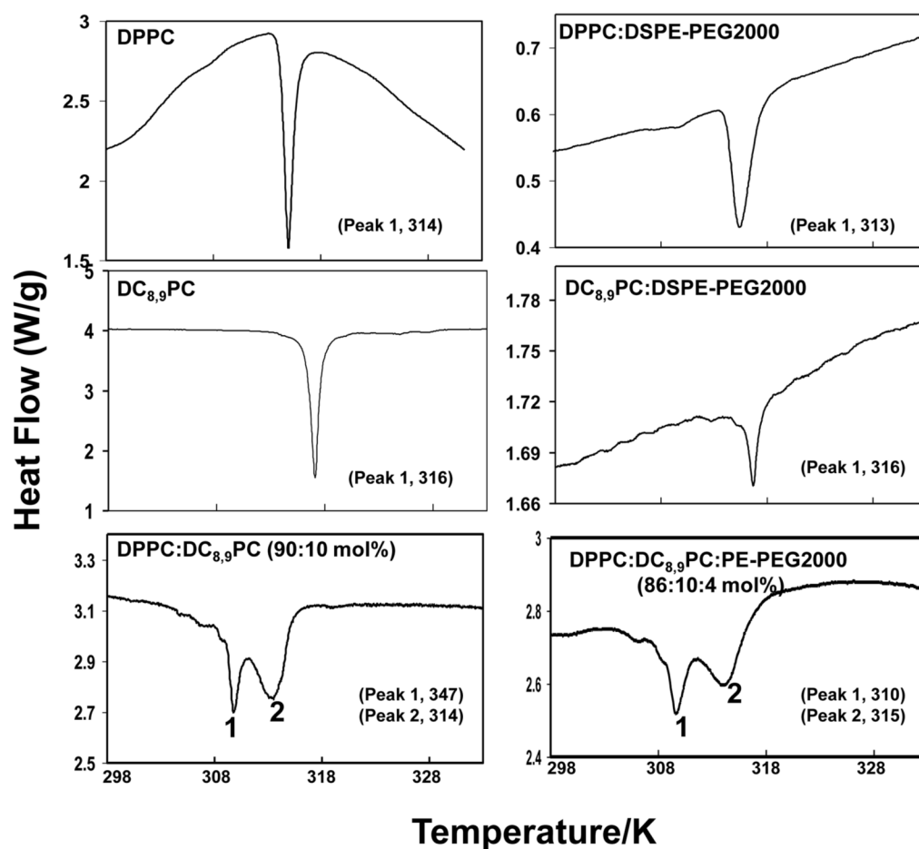
Figure 3. Differential scanning calorimetry (DSC) of DPPC and DC 8,9 PC dispersions Cooling cycles of curves of aqueous dispersions of pure lipids and lipid mixtures (1–2 mg) were recorded (Methods section). The phase transition peaks of individual lipids are indicated in the respective graphs. Left panels show without the inclusion of DSPE-PEG2000. Right panels show the effect of inclusion of 4 mol% DSPE-PEG2000 on T m of DPPC, DC 8,9 PC or the lipid mixtures.
