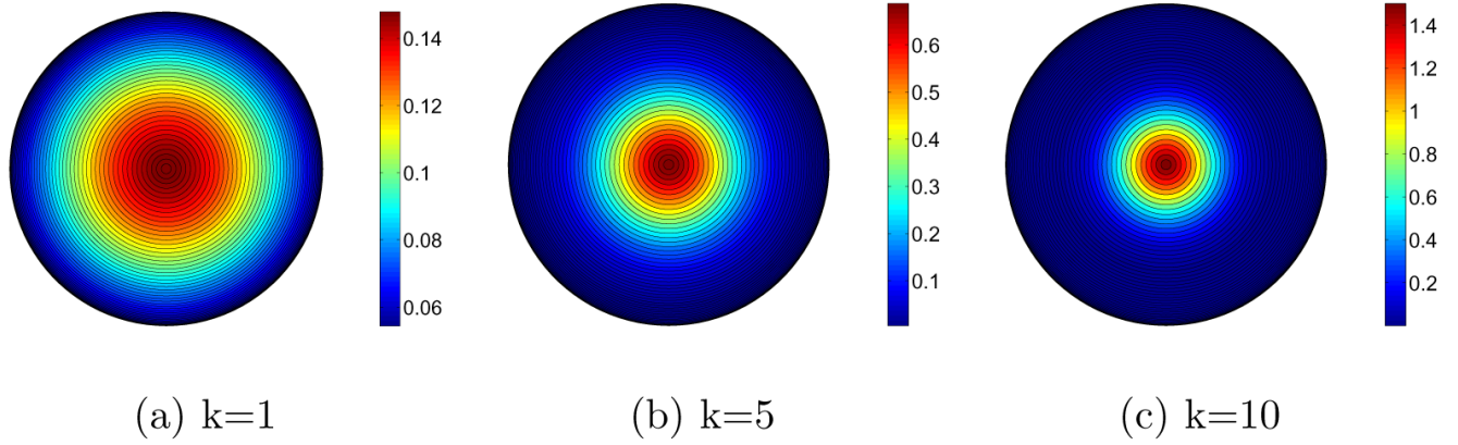
Fig. 8. Watson distributions projected along direction \mu onto the unit disk for a sample of concentration parameters k .
