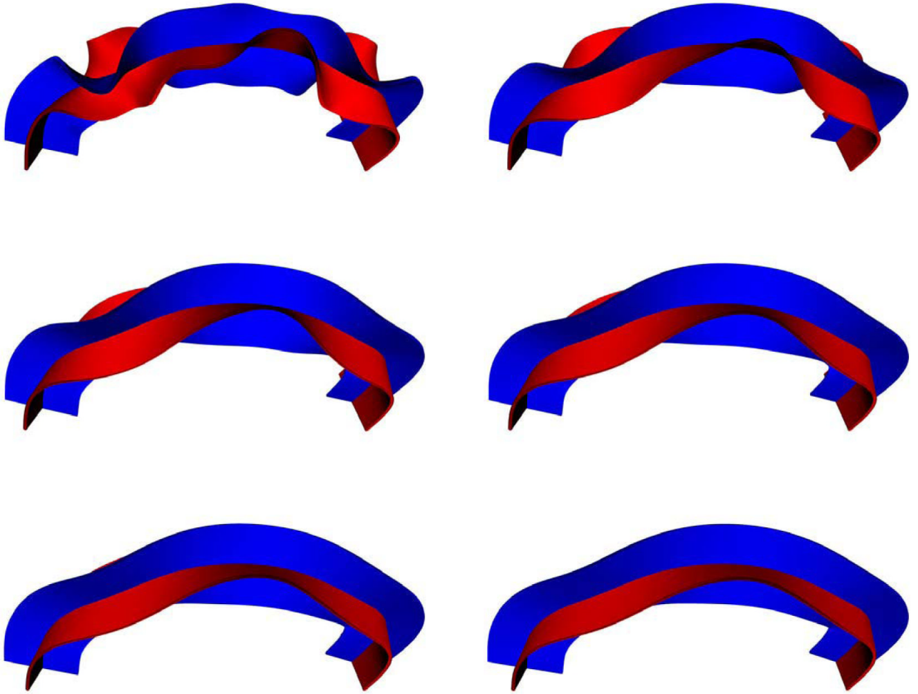
Fig. 5. Regularization of the Frenet frame with tangential direction fixed helps obtaining smoothly varying frames from noisy data on a space curve.
