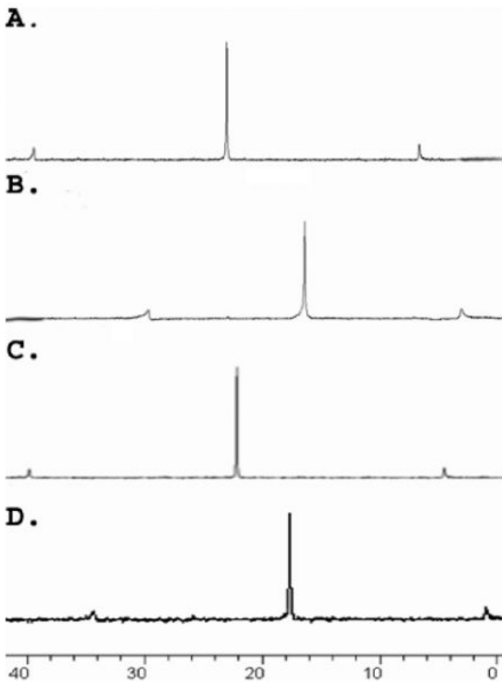
Figure 1. ^{31}\text{P} NMR spectra (300 MHz, \text{CD}_2\text{Cl}_2 , 298 K) of (A) acceptor 1 , (B) cuboctahedron 4 , (C) acceptor 2 , and (D) cuboctahedron 5 .
