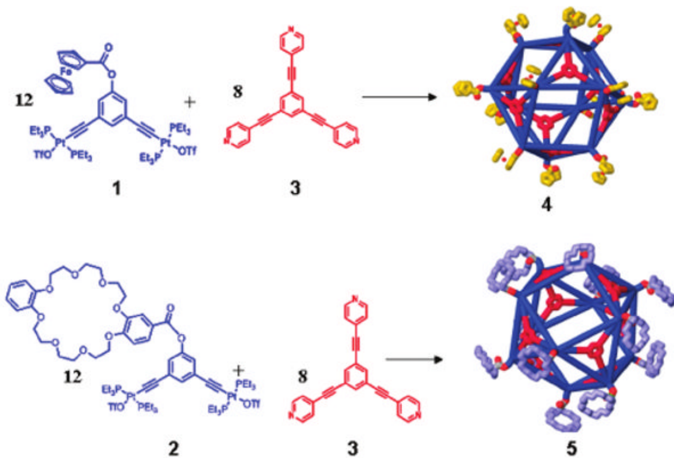
Scheme 1. Graphical Representation of the Self-Assembly of Cuboctahedra 4 and 5
