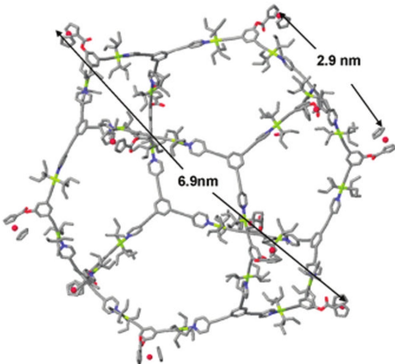
Figure 2. Molecular modeling of multiferrocenyl cuboctahedron 4 .
