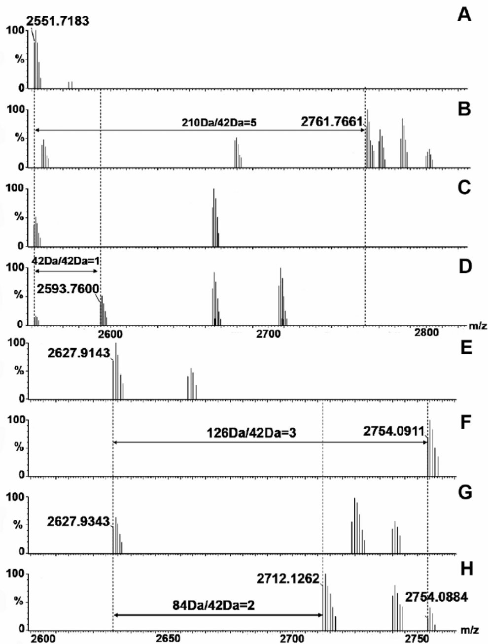
Fig. 4. MALDI spectra of peptide fragment NKPAAKTDATIKKEQKLIQAQNL (95-117, m/z 2551, A-D) and fragment FEKTHTVSAHRKAQKAVNLVSFE (120-143, m/z 2627, E-H) of Efb(-C) derived from samples A) free Efb-C without lysine acetylation; B) free Efb-C with lysine acetylation; C) Efb-C/C3d without lysine acetylation; and D) Efb-C/C3d with lysine acetylation. The mass differential of 168 Da (210 Da - 42 Da) in the free protein versus the protein complex indicated that 4 lysine residues in Efb-C were protected upon Efb-C/C3d binding; E) free Efb-C without lysine acetylation; F) free Efb-C with lysine acetylation; G) Efb-C/C3d without lysine acetylation; and H) Efb-C/C3d with lysine acetylation. The mass
