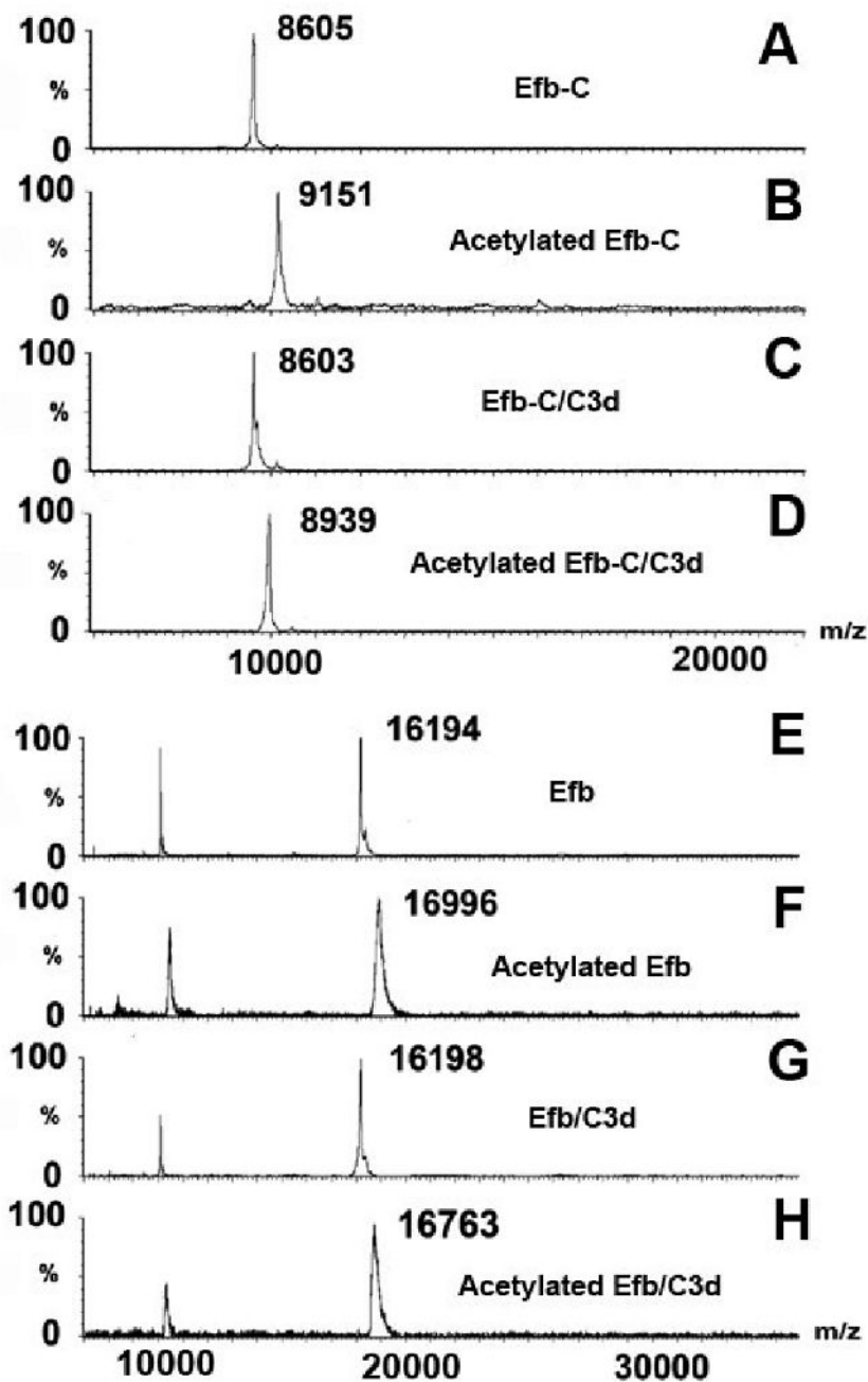
Fig. 3. MALDI spectra of Efb-C (A-D) and Efb (E-H) under linear mode. Sample identities are A) free Efb-C without lysine acetylation; B) free Efb-C with lysine acetylation; C) Efb-C/C3d without lysine acetylation; and D) Efb-C/C3d with lysine acetylation; E) free Efb without lysine acetylation; F) free Efb with lysine acetylation; G) Efb /C3d without lysine acetylation; and H) Efb /C3d with lysine acetylation. The mass differential between sample A and B was 546 Da = 9151-8605, indicating that 13 lysine residues were acetylated in the free protein sample. In contrast, the 336 Da (= 8939-8603) difference between complex samples C and D demonstrated that only 8 lysine residues were labeled. The differential labeling between free
