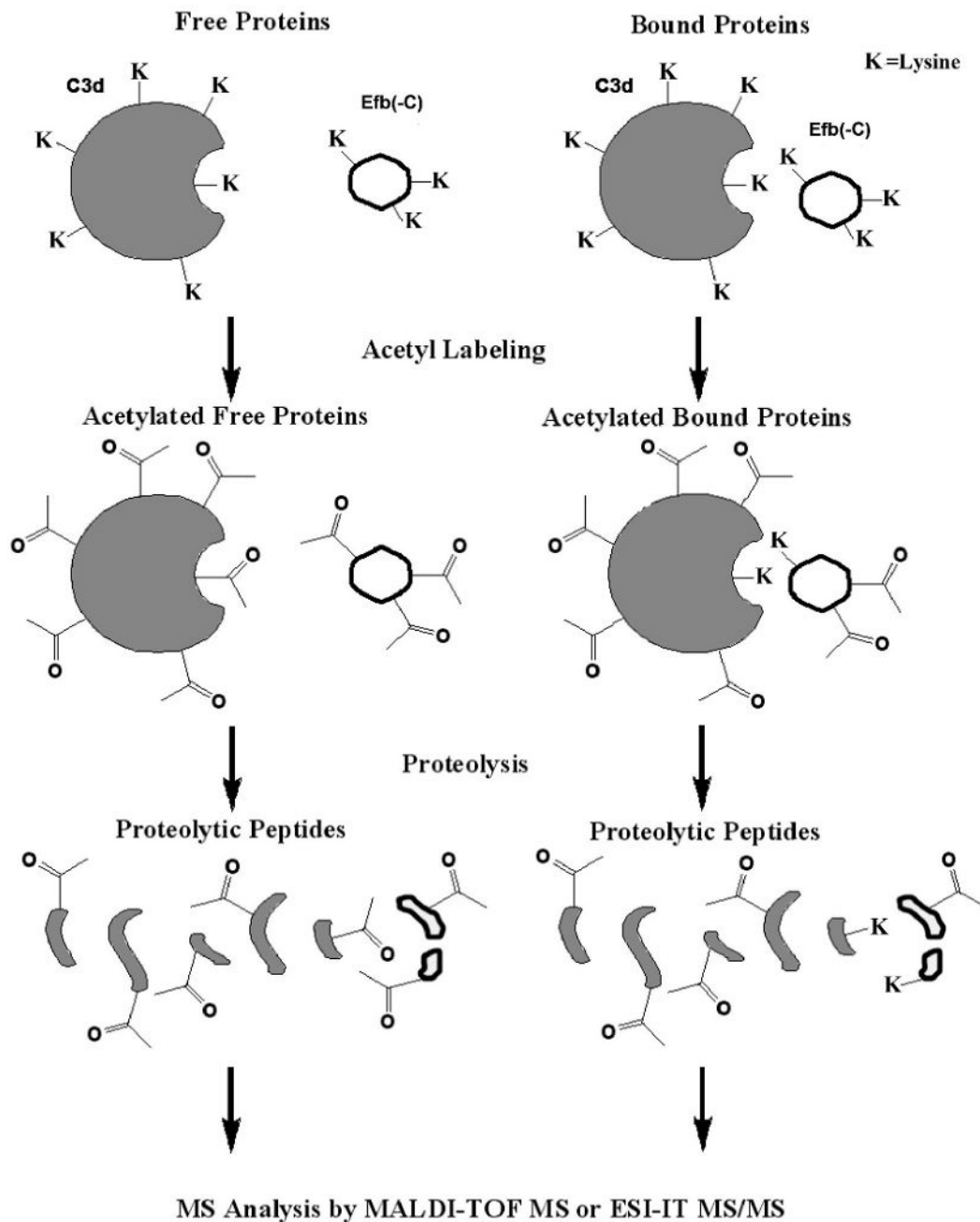
Fig. 1. Brief scheme of experimental labeling procedure. C3d (in dark color), Efb(-C) (in light color) or their complex are labeled using the lysine acetylation reagent. After 20 minutes at room temperature, the acetylation reaction is quenched by addition of \text{NH}_4\text{HCO}_3 and followed by proteolytic digestion. Both chymotrypsin and glutamic-C V8 were used to achieve the most complete peptide coverage maps.
