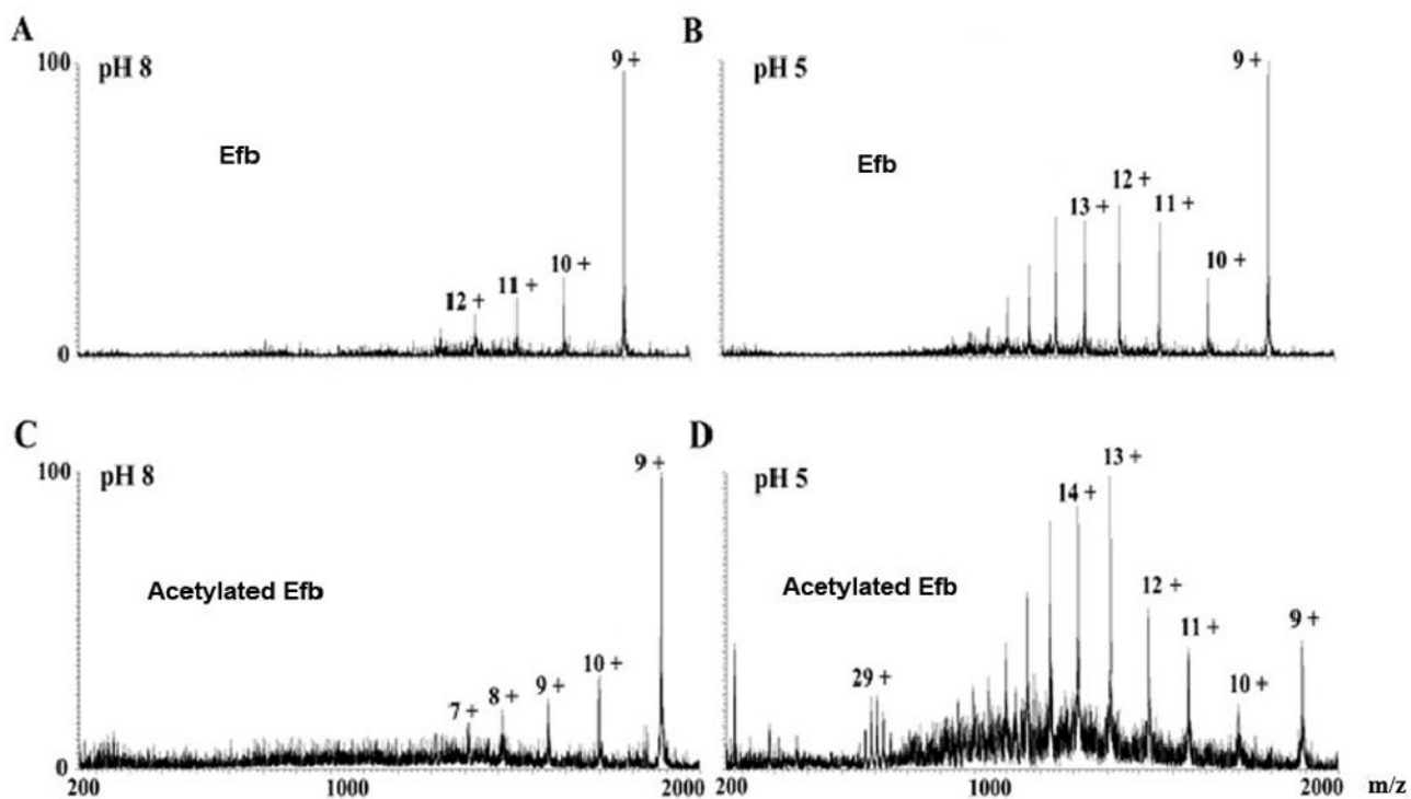
Fig. 2. ESI mass spectra of Efb and acetylated Efb recorded at different pH values. A) Efb at pH 8; B) Efb at pH 5; C) acetylated Efb at pH 8, D) acetylated Efb at pH 5. Peaks are labeled according to the corresponding charge states. Note that acetylated Efb displayed the same charge state distribution as native protein at multiple pH values. Similar results were obtained in an ESI charge state distribution analysis of Efb-C (see supplemental figure 1). This suggested that the acetylation reaction itself did not perturb the folding state of Efb(-C).
