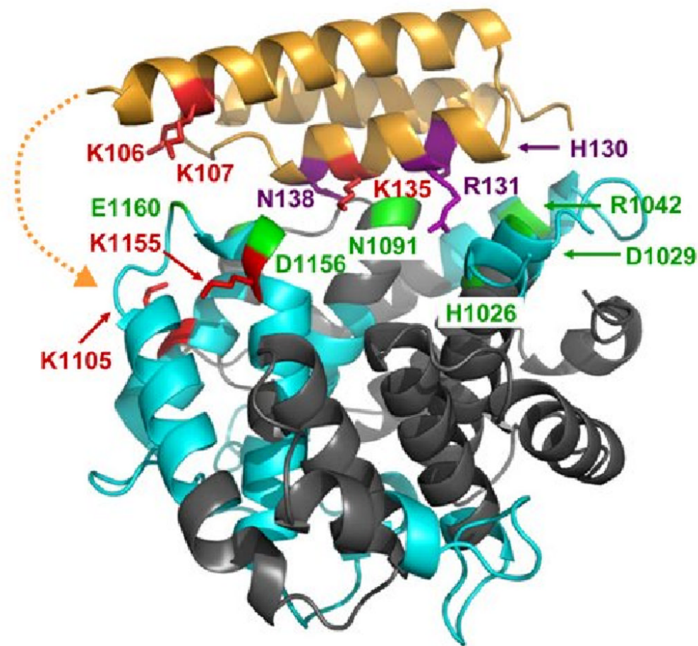
Fig. 6. Interaction sites of C3d binding to Efb(-C) as determined by differential lysine acetylation. Efb-C is drawn as in Fig. 6, while C3d is shown in ribbons colored according to regions of peptide coverage as described in Table 2 (blue ribbon) and uncovered regions (slate). Selected contacting residues of C3d which bind to Efb-C according to x-ray crystallography are shown in green. These are H1026, D1029, R1042, N1091, S1097, D1156 and E1160. K1155 in fragment ISLQEAKDICEEQ VNSLPGSITKAGDFL (1149-1176) was protected in Efb-C/C3d, implying that D1156 may contact Efb-C. In addition, K1105 in fragment CGAVKWK (1101-1106) was protected from acetylation in the complex. This suggested that portions of Efb(-C) not present in the crystal structure model may also be contacting C3d near residue K1105. The potential location for additional contacts invisible in the Efb-C/C3d crystal structure is depicted by a dashed orange line. No evidence was obtained regarding the role of R1042 in the Efb-C/C3d complex, since K1041 in fragment GLEKRQ GAL (1038-1046) was solvent accessible in the complex. Similarly, no further information was available for H1026, D1029 and N1091, as no identified peptides covered this sequence, nor were there any lysine residues in these regions.
