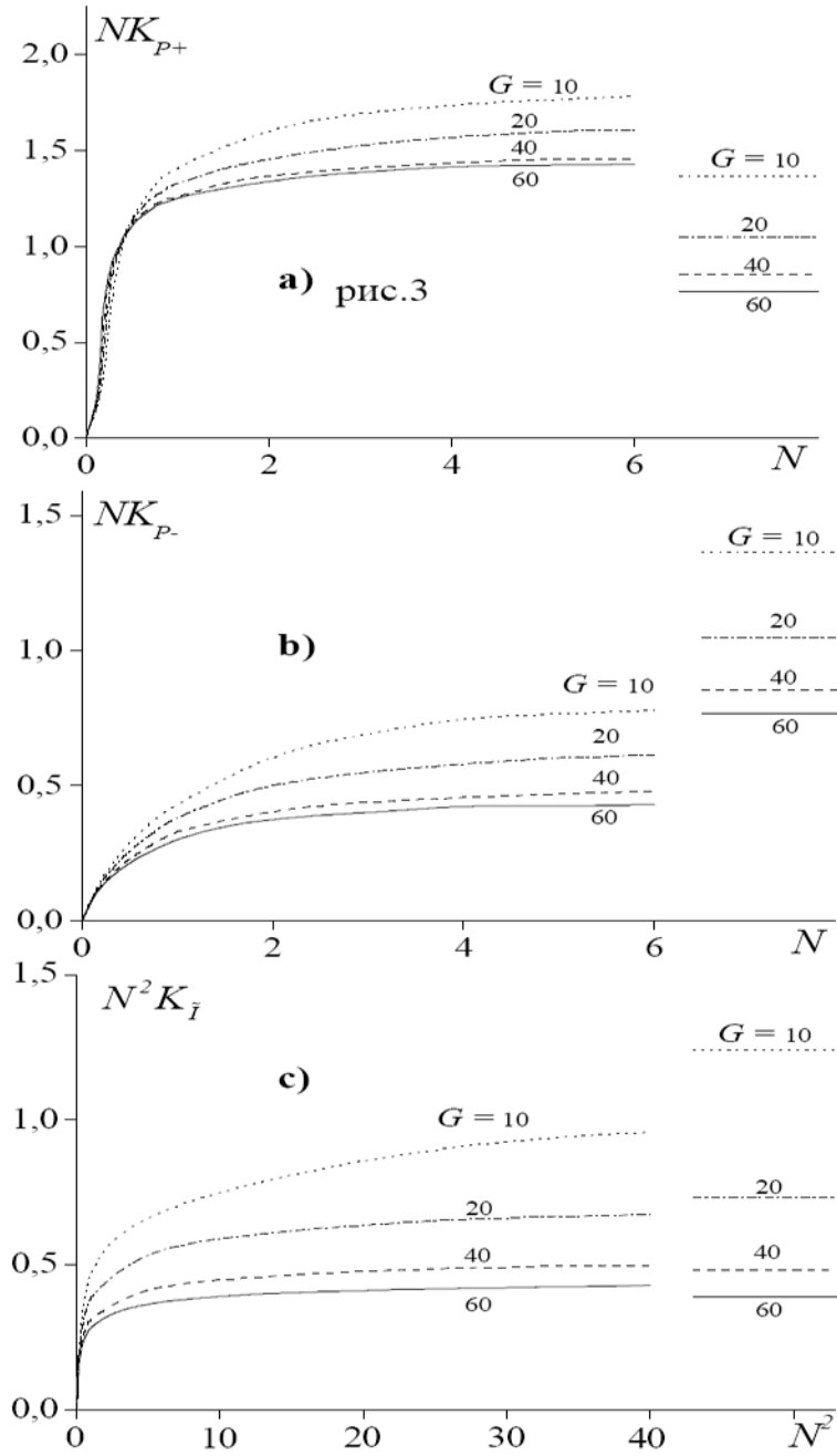
FIG. 3. Saturation curves at the focus for dimensionless peak pressures ( NK_{P_{\pm}} \sim p_{\pm}^F , a, b) and intensity \tilde{I} (N^2 K_{I} \sim I^F , c). The value of parameter N is proportional to the source pressure output p_0 , the curves are presented for various values of G = 10, 20, 40, 60 . Shown on the right are the approximate saturation values given by the analytic solution, Eq. 5.
