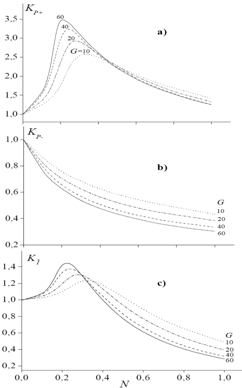
FIG. 2. Dependences of correction factors to the focusing gains in nonlinear beam on nonlinear parameter N for the peak positive p_+^F (a) and peak negative p_-^F (b) pressures, and intensity I^F (c). Correction factors are defined as K_{P+} = p_+^F/p_0G , K_{P-} = p_-^F/p_0G , and K_I = I^F/I_0G^2 , where G is the linear focusing gain of the source ( G = 10, 20, 40, 60 ).
