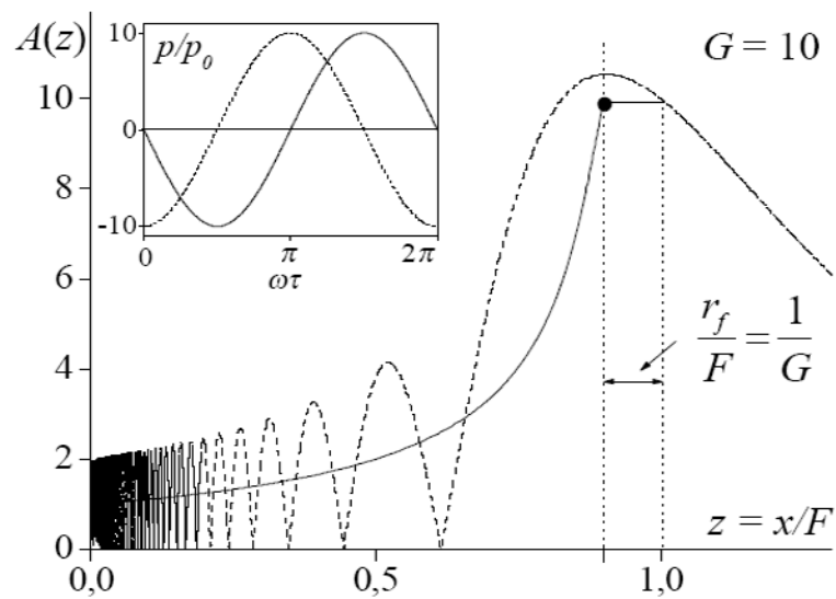
FIG. 1. Distributions of the dimensionless amplitude of harmonic wave along the axis z = x/F of the piston transducer for 1D spherically convergent wave (solid line) and linear focused beam (dashed line) with the focusing gain G = 10 . The waveforms of the same amplitude are shown in the small figure (for linear focused beam - in the geometrical focus, for 1D spherical convergent wave - at the distance z = 1/G prefocally).
