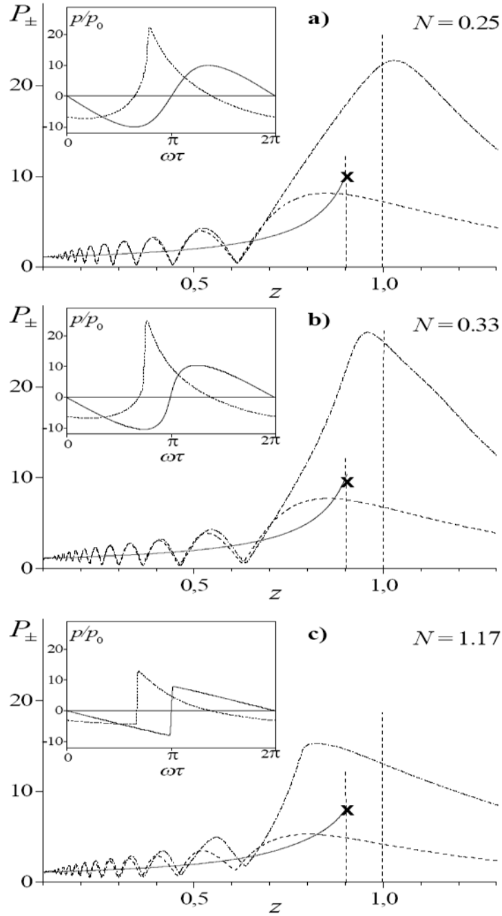
FIG. 5. Distributions of the dimensionless peak pressures P_+ and P_- along beam axis ( G = 10 ) for various values of nonlinear parameter N = 0.25 (a), 0.33 (b), and 1.17 (c). Solid lines correspond to the peak pressure in one-dimensional spherically convergent wave ( P_+ = P_- ); dashed lines – to the peak negative P_- and dash-dotted line – to the peak positive P_+ pressure in nonlinear beam. Shown in small frames are waveforms calculated in the geometrical focus for a beam and at the distance 1/G from the focus towards the source for one-dimensional spherically convergent wave.
