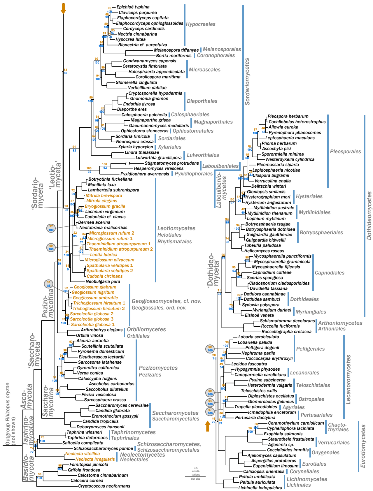
Fig. 2 A most likely tree obtained by RAxML for Ascomycota (as in Fig. 1). Phyla, subphyla, class, order and rankless taxa are indicated. Taxa designated as earth tongues are indicated in orange. The tree is displayed as two subtrees – orange arrows indicate where the subtrees were joined. The tree was rooted with outgroup Rhizopus oryzae (not shown). Bootstrap values are shown in orange above nodes and Bayesian posterior probabilities in blue below. Numbers were removed for nodes with 100 % bootstrap and 100 % posterior probability.
