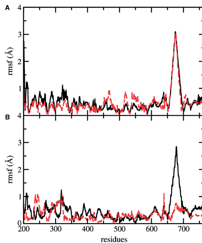
Figure 7. Displacements of each C\alpha atom along the first two eigenvectors are represented in black continuous lines and dashed red lines for the wild type and Lys681Ala mutant, respectively. (A) Displacements along the first eigenvector. (B) Displacements along the second eigenvector.
