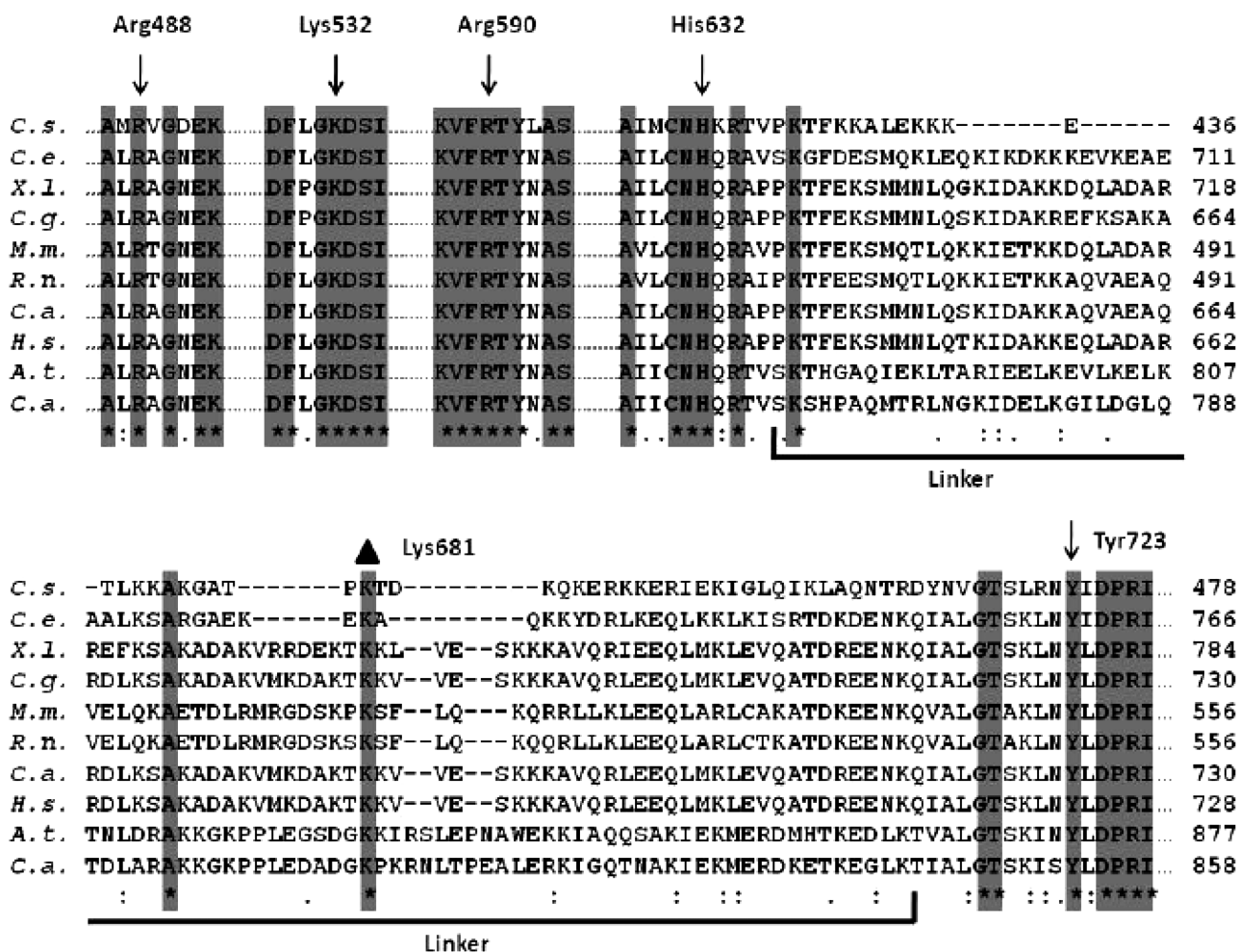
Figure 1. Multiple sequence alignment of the topoisomerase IB sequences extracted from C. symbiosum , C. elegans , X. laevis , C. griseus , M. musculus , R. norvegicus , C. aethiops , H. sapiens , A. thaliana and C. acuminata , respectively. The alignment of the residues in proximity of the catalytic pentad (Arg488, Lys532, Arg590, His632, Tyr723 for the human isoform) and along the full linker domain is reported. Residues conserved in all sequences are highlighted by a grey column and evidenced by an asterisk. The residues belonging to the linker domain are underlined. The mutated residue Lys681 is evidenced by a black triangle.
