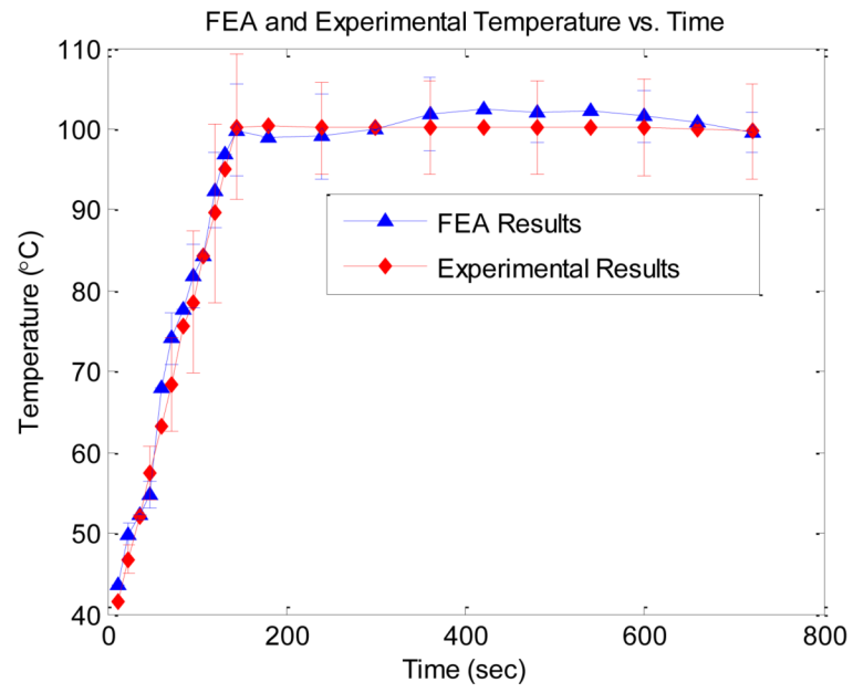
Figure 2. Comparison of the average time temperature versus time for an actual experimental results and an FEA simulation.
