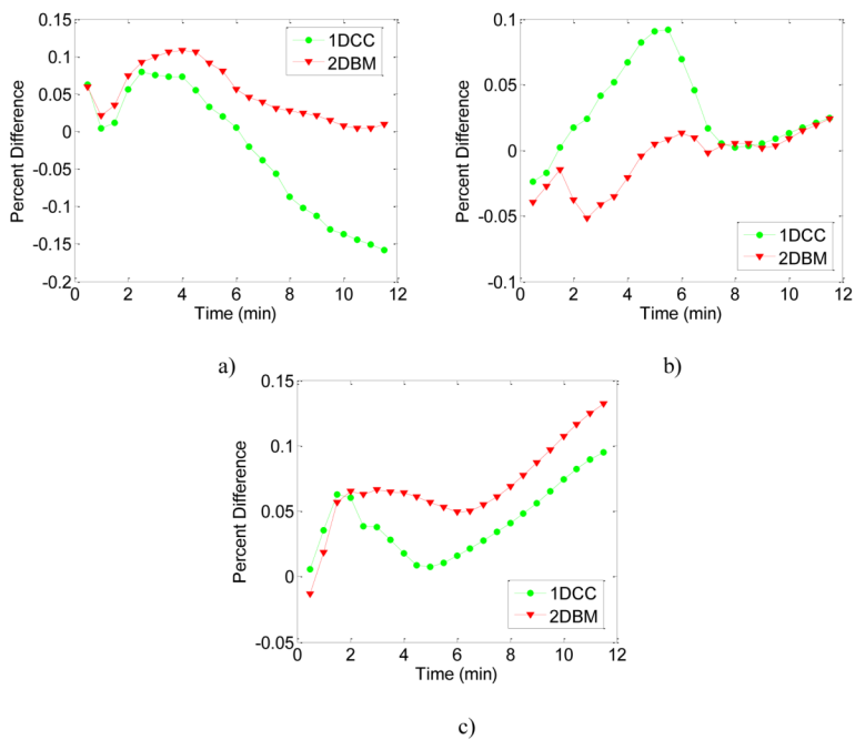
Figure 9. Comparison of the percent difference or error between temperature estimates calculated using 1D CC and 2D BM based temperature algorithms using the calibration curve versus the “ideal” FEA temperature. The red curve denotes 2D BM and the green curve 1D CC results. The percent difference in temperature was computed for the three ROI shown in Figure 8, at the a) tine (left side), b) simulated liver (right side) and at the d) center.
