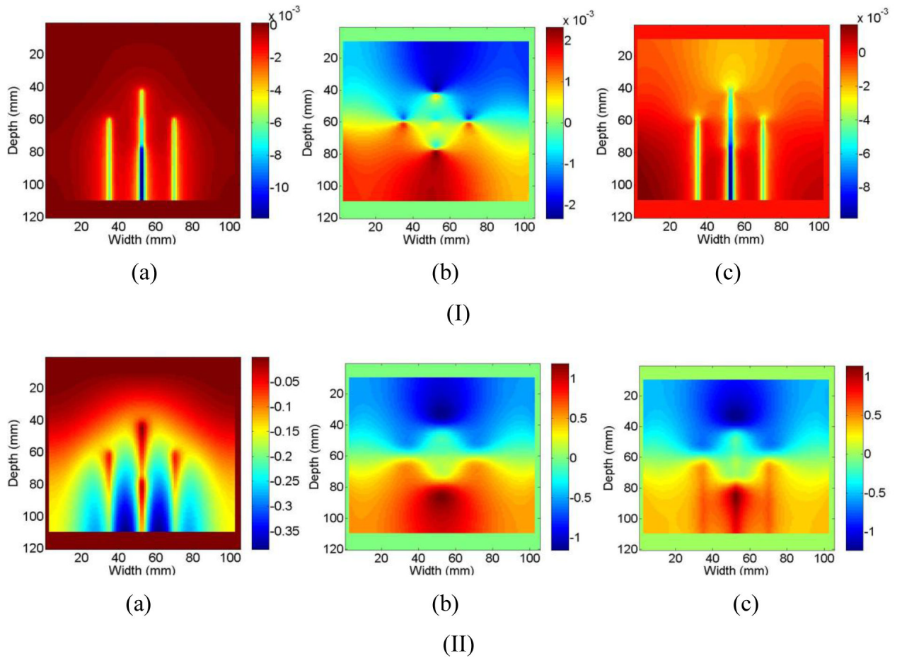
Figure 4. Ideal displacement images due to a) SOS changes, b) thermal expansion and c) cumulative displacements after I) 6 seconds and II) 360 seconds after ablation.
