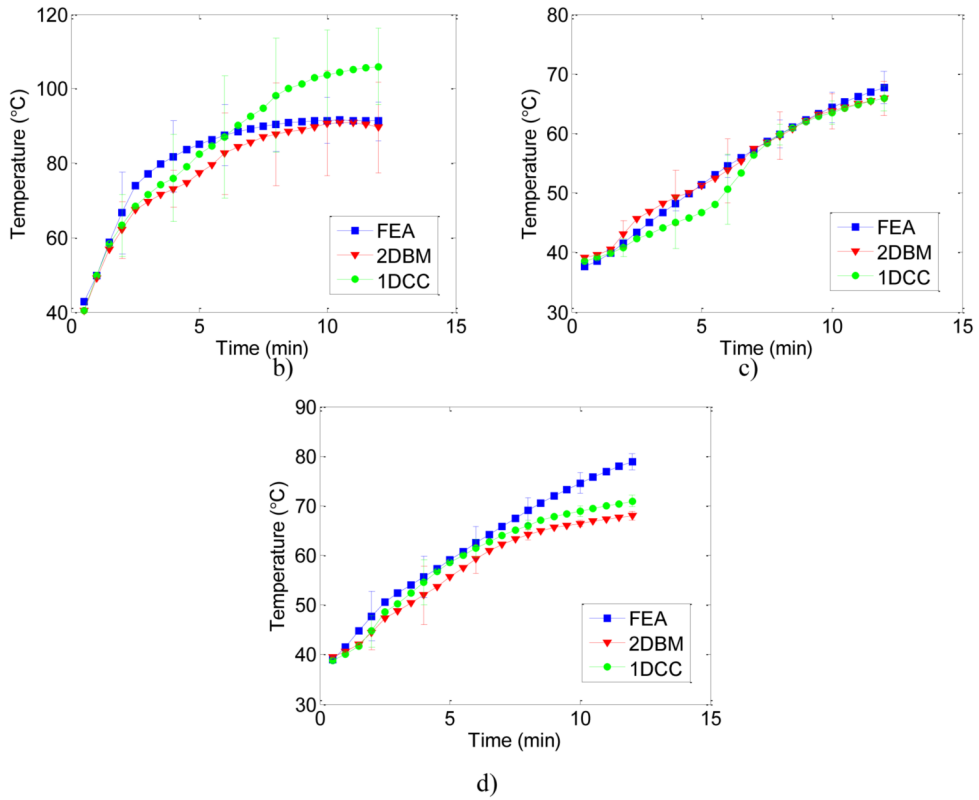
Figure 8. FEA temperature images illustrating the regions of interest (ROI) over which the temperature estimates obtained using FEA and US simulations based on 1D CC and 2D BM algorithms were compared in Figure 8 a). Quantitative comparisons of the temperature estimated from ultrasound simulation using the 1D CC and 2D BM based temperature estimation algorithms using the calibration curve. The blue curve denotes the FEA computation, the red curve 2D BM and the green curve 1D CC results. Displacement data was accumulated from radiofrequency echo data acquired every 6 seconds for ROI's at the b) tine (left side), c) simulated liver (right side) and at the d) center. The errorbars are shown only for limited estimates to reduce the clutter in the graph.
