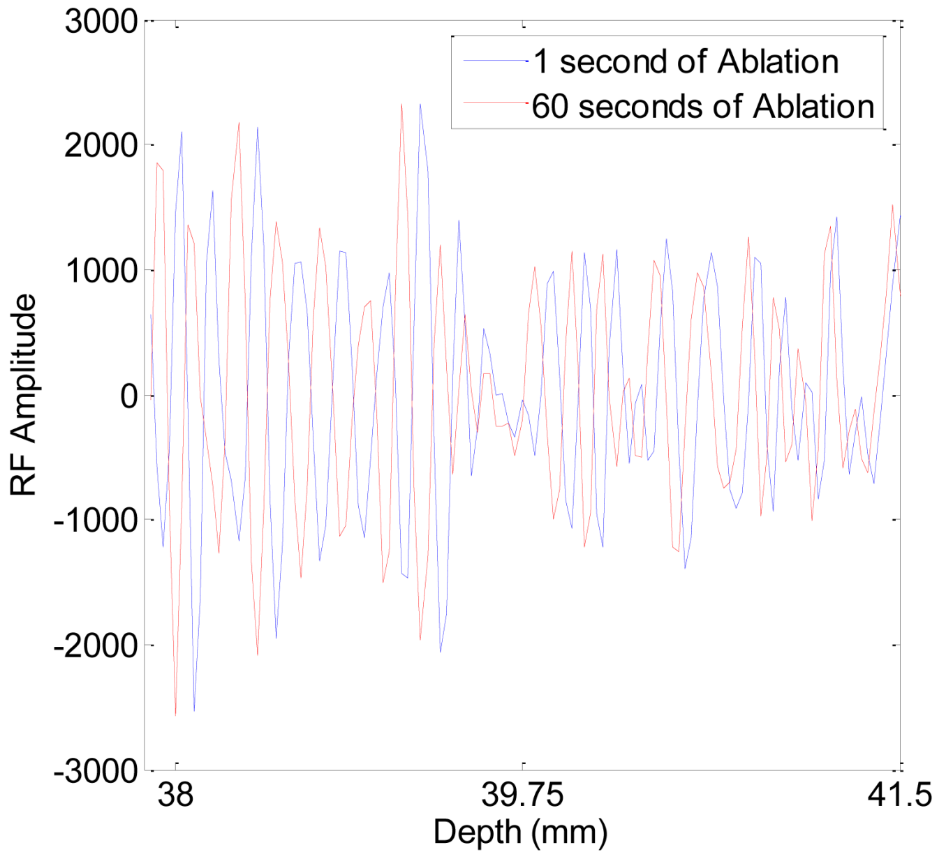
Figure 5. Radiofrequency echo data segment near the upper tine after 1 second (blue) and 60 seconds (red) of ablation.
