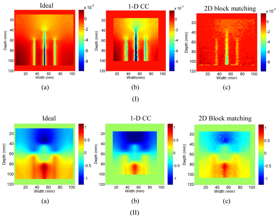
Figure 6. Comparison of the a) ideal total displacement obtained using FEA to the b) 1D and c)2D BM accumulated displacement, after I) 6 seconds and II) 360 seconds after ablation.
