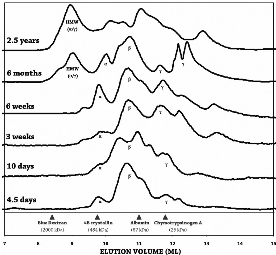
Figure 1. Size exclusion chromatography of zebrafish lens homogenates during development and aging. Absorbance at 280 nm for detection of proteins was plotted versus elution volume (x-axis), which corresponds with molecular size. Individual protein molecular weight standards are shown at the bottom of the graph. High molecular weight aggregates elute early followed by a broad peak of polydisperse \alpha -crystallin oligomers with an average size of 24 subunits. Next, a broad peak of \beta -crystallin elutes from the column, which forms octamers, tetramers, and dimers, and finally, \gamma -crystallins, which are monomeric, were observed. The youngest lenses (4.5 days) were dominated by a large broad \beta -crystallin peak. \alpha -Crystallin and \gamma -crystallin abundance increased during lens maturation, and a high molecular weight peak, first observed at six months, increased with age to become the largest peak by 2.5 years.
