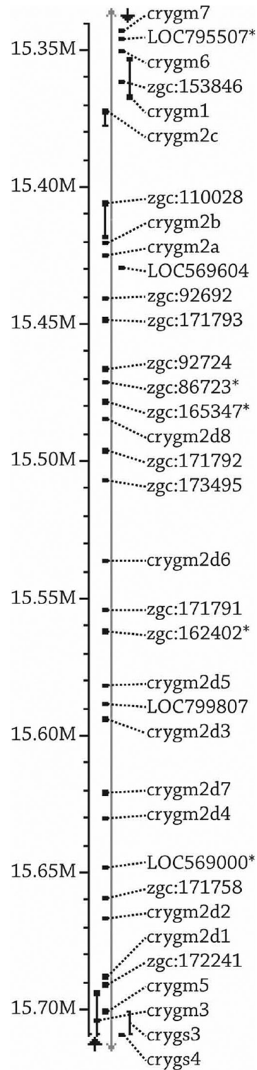
Figure 5. Zebrafish chromosome 9,400 kilobase-pair region containing 35 known and hypothetical \gamma M-crystallin genes. Proteins from 30 genes in this region were found by shotgun proteomic analysis of the zebrafish lens (Table 3). The five genes marked (indicated by asterisk) were not detected but also show sequence similarity to the \gamma M-crystallins. Gene positioning was determined by the NCBI map viewer , Ensembl Genes on Sequence Map . The scale on the left side of the image represents mega base-pairs. The gray line represents the chromosome. Genes on the left side of the gray line are located on the minus strand, and genes on the right side of the gray line are located on the plus strand.
