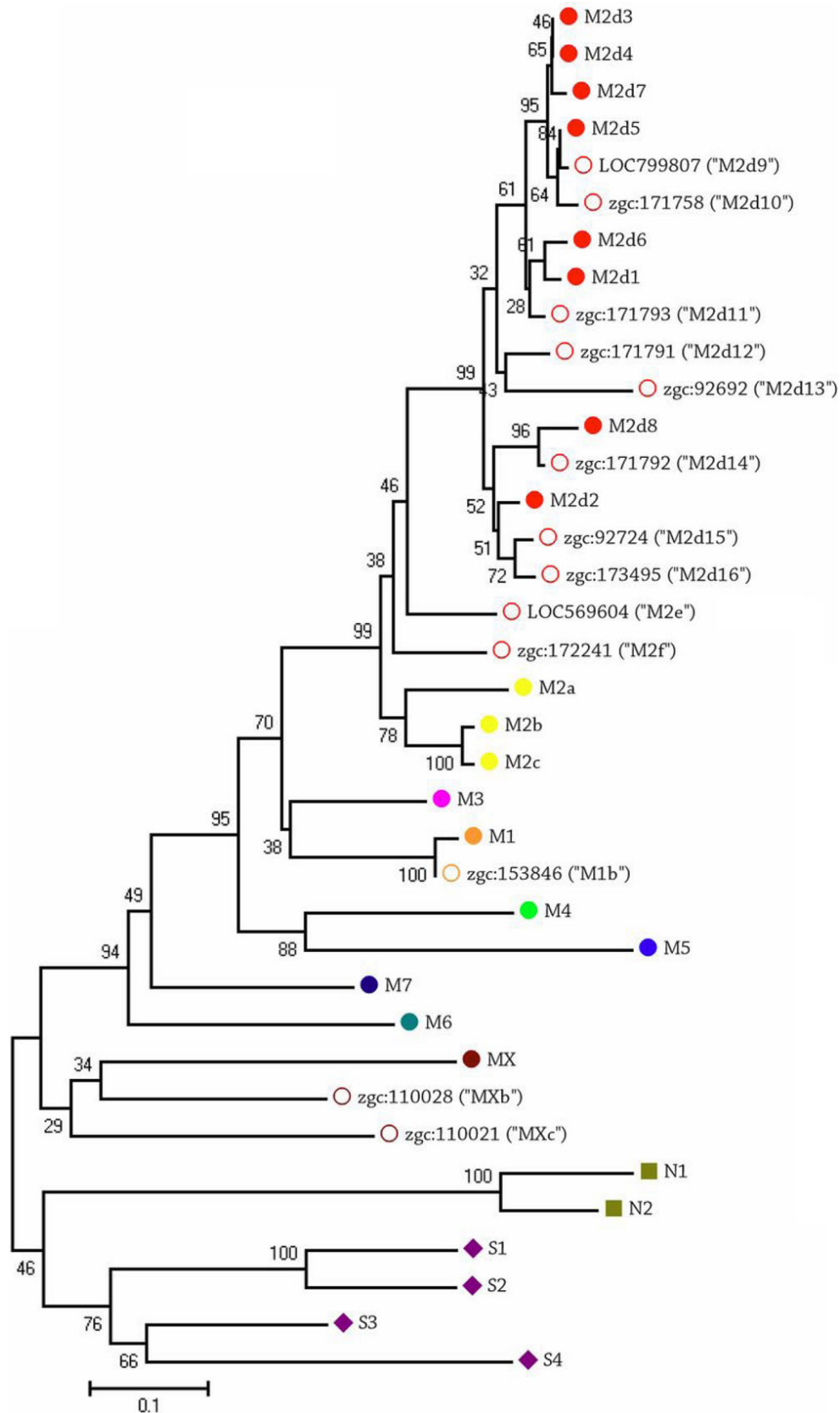
Figure 4. Phylogenetic tree of zebrafish \gamma -crystallin genes constructed by Mega 4 with 1000 bootstraps. All zebrafish \gamma -crystallins listed were detected by shotgun proteomics of the zebrafish lens (Table 3). Thirteen novel \gamma -crystallins (unfilled symbols) were detected and named based on their alignment.
