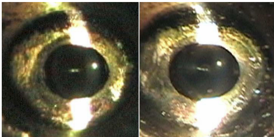
Figure 2. Slit-lamp views of living, anesthetized six-month-old (left panel) and 2.5-year-old (right panel) WIK zebrafish. Minimal light scattering is visible from the cornea, and no light scatter is visible from the lens. Lens transparency was maintained over 2.5 years, demonstrating the clarity of the lens and cornea in the zebrafish at ages up to 2.5 years.
