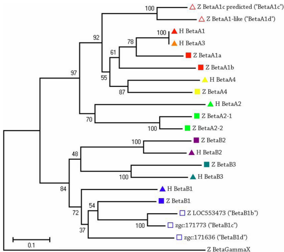
Figure 3. Phylogenetic tree of human and zebrafish \beta -crystallin genes constructed by Mega 4 with 1000 bootstraps. All zebrafish \beta -crystallins listed were detected by shotgun proteomics of the zebrafish lens (Table 2). Five novel \beta -crystallins (unfilled symbols) were detected and named based on their alignment. H, human; Z, zebrafish.
