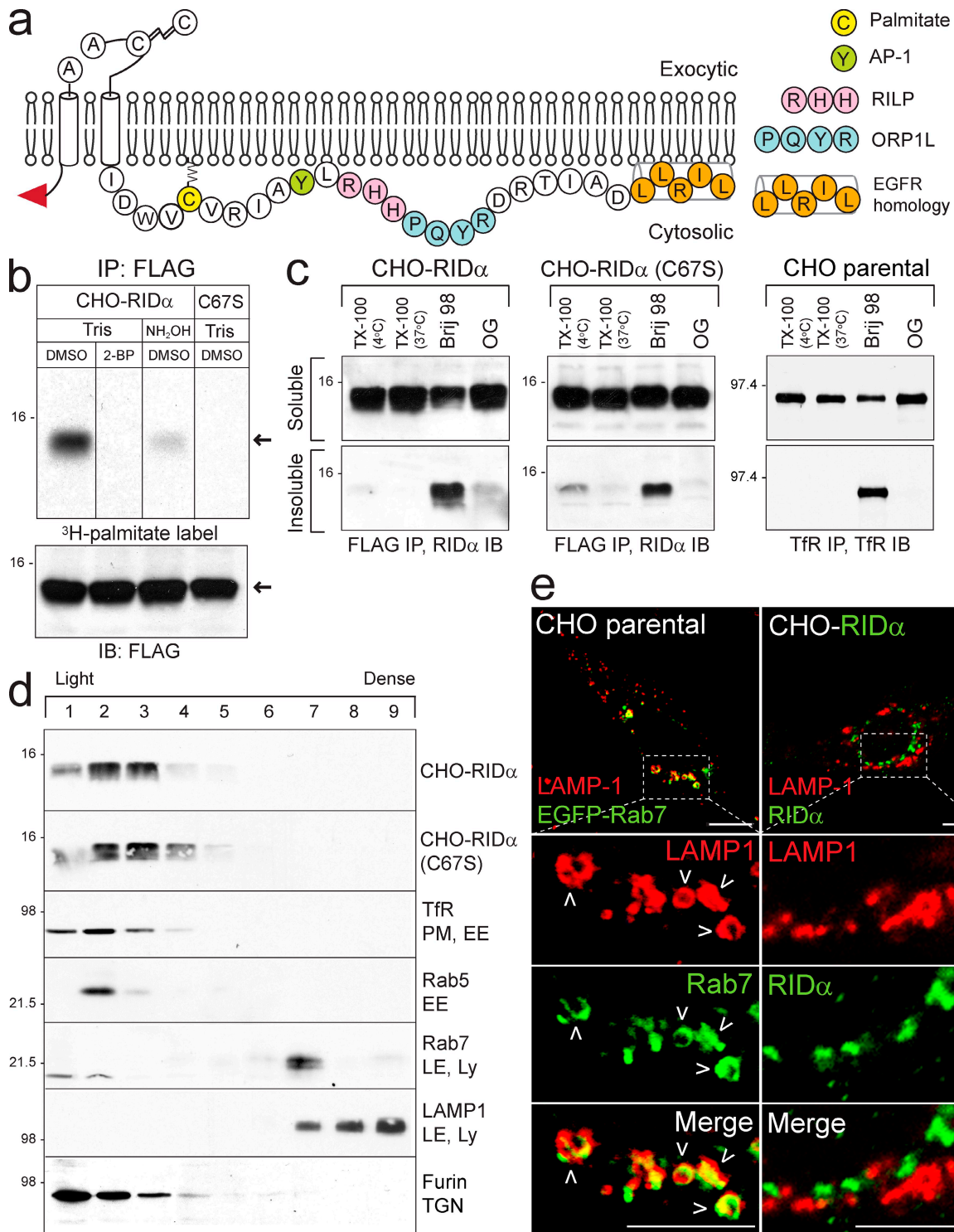
Figure 2. RID- \alpha is palmitoylated at Cys67. (a) Schematic of RID- \alpha membrane topology showing the amino-terminal Flag epitope (red arrowhead), luminal signal peptidase cleavage (which generates 13.7- or 11.3-kD RID- \alpha species) and disulfide bond formation sites, carboxyl tail sequence with palmitoylation and protein interaction sites, and the EGFR homology domain (Hoffman et al., 1992b; Vinogradova et al., 1998; Tsacoumangos et al., 2005; Cianciola et al., 2007; Shah et al., 2007). (b) CHO-RID- \alpha and CHO-RID- \alpha (C67S) cells treated with 2-BP or DMSO and radiolabeled with [ 3 H]palmitate. Flag immunocomplexes were separated by SDS-PAGE, and gels were incubated with Tris or hydroxylamine solutions before fluorography. The bottom panel shows Flag immunocomplexes from duplicate samples analyzed by RID- \alpha immunoblotting for loading control. Arrows denote 13.7-kD and RID- \alpha species. (c) CHO cell lines extracted with the indicated detergents and RID- \alpha (left and middle) or TfR (right) immunocomplexes from detergent-soluble and -insoluble fractions immunoblotted with antibodies to the same protein. (d) Membranes from stable CHO cells expressing wild-type RID- \alpha or RID- \alpha (C67S) fractionated on 27% Percoll gradients and equal aliquots of total membrane protein immunoblotted with antibodies to RID- \alpha (top two panels) are shown. Equal aliquots of total membrane protein from parental CHO cells immunoblotted with antibodies to marker proteins for intracellular membrane compartments listed in the figure (bottom five panels) are shown. (b–d) Molecular mass is indicated in kilodaltons. (e) Confocal images of CHO cells transfected with EGFP-Rab7 plasmid and stained for LAMP1 or CHO-RID- \alpha cells stained for LAMP1 and RID- \alpha . Boxed areas show regions of the image that were magnified. Arrowheads denote compartments with colocalized markers. IB, immunoblot; IP, immunoprecipitation; Ly, lysosome; OG, octyl glucoside; TX-100, Triton X-100. Bars, 10 \mu m.
