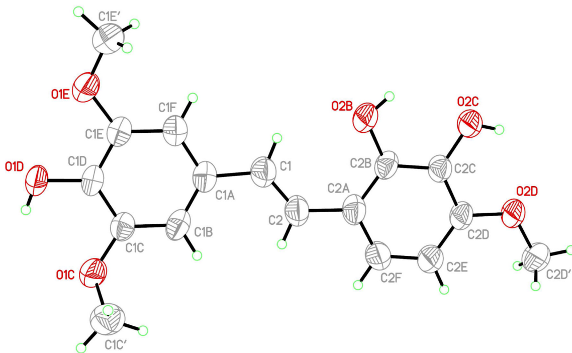
Figure 1. X-ray crystal structure of E -stilstatin 3 ( 3a ).
