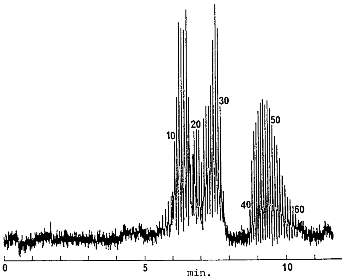
Figure 1. Capillary gel electrophoresis separation of polydeoxyadenylic acids, p(dA)_{10-30,40-60} . Capillary: 270 \times 0.075 mm i.d.; running buffer: 0.1 M Tris/0.25 M borate/7 M urea, pH 8.3, with crosslinked polyacrylamide gel: 7.5% T and 3.3% C. The applied electric field was 400 V/cm. With permission from [8].
