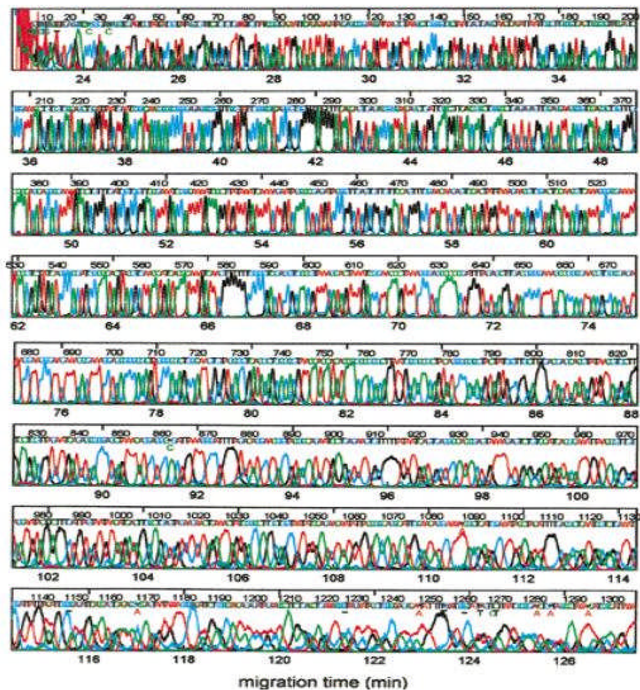
Figure 4. Sequencing to 1300 bases at 70°C using high molecular mass polymer matrix, optimized electric field and base calling software. With permission from [35].
