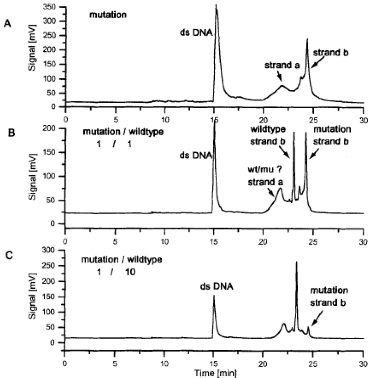
Figure 2. Comparison of the migration behavior of wild-type and mutated DNA strands of luc1 gene. With permission from [21].
