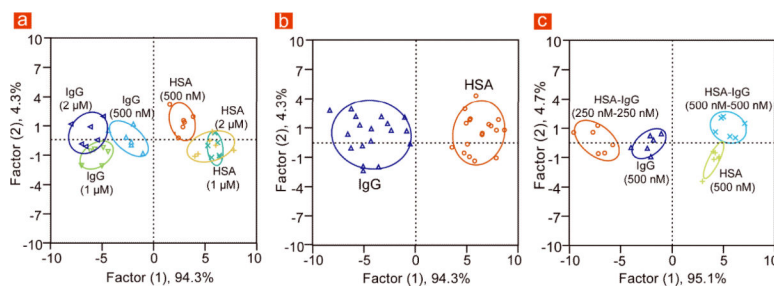
Figure 5. Discrimination of HSA and IgG at different concentrations and mixture of proteins (a) Canonical score plot for the fluorescence patterns as obtained from LDA for human serum albumin (HSA) and immunoglobulin G (IgG) at different concentrations (500 nM, 1 \mu M and 2 \mu M) with 95% confidence ellipses. (b) Clustering of all the data for the three concentrations mentioned for each protein as obtained from LDA analysis. (c) HSA and IgG were mixed at 1:1 molar ratio with 250 nM each and 500 nM each and added to five GFP-NP complexes. The canonical score plots obtained from LDA analysis were compared with that for the 500 nM of the individual proteins.
