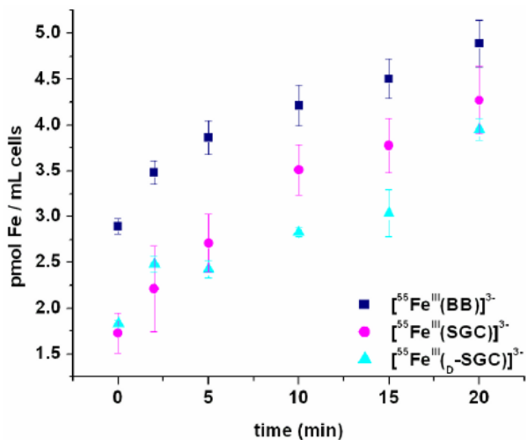
Figure 4. Iron transport mediated by [^{55}\text{Fe}^{\text{III}}(\text{BB})]^{3-} , [^{55}\text{Fe}^{\text{III}}(\text{SGC})]^{3-} , and [^{55}\text{Fe}^{\text{III}}(\text{b-SGC})]^{3-} in B. subtilis at 37 °C in iron-limited medium. Data presented are the average of three independent experiments for BB and SGC, and two independent experiments for b-SGC.
