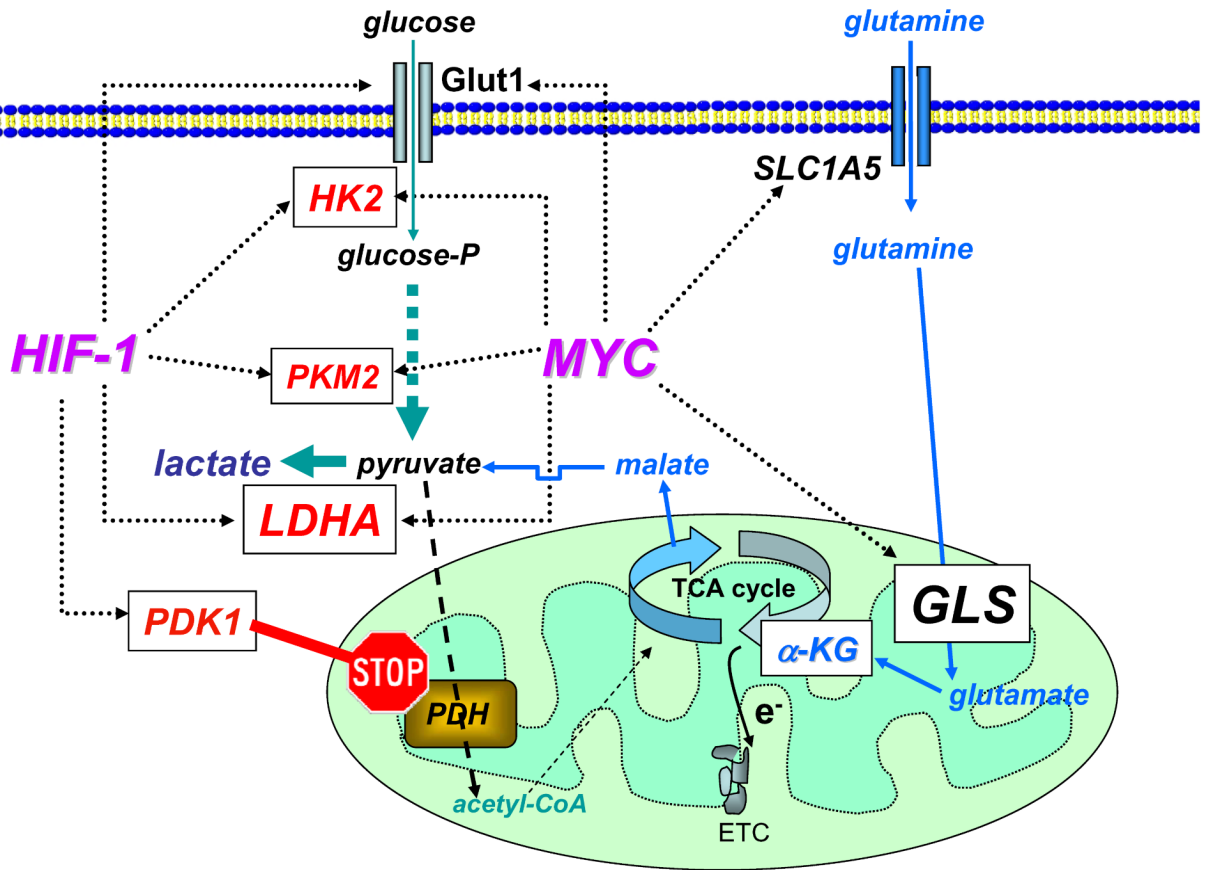
Figure 2. Myc and HIF-1 regulate glucose metabolism and stimulate the Warburg effect Myc and HIF-1 are depicted to regulate (dotted lines) genes involved in glucose metabolism (glucose transporter Glut1, hexokinase 2 (HK2), pyruvate kinase M2 (PKM2), lactate dehydrogenase A (LDHA), and pyruvate dehydrogenase kinase 1 (PDK1)), favoring the conversion of glucose to lactate (glycolysis). Myc is also depicted to stimulate glutamine metabolism through the regulation of transporters (SLC1A5) and glutaminase (GLS). Glutamine is shown converted to \alpha -ketoglutarate ( \alpha -KG) for catabolism through the tricarboxylic acid (TCA) cycle to malate, which is transported into the cytoplasm and converted to pyruvate and then to lactate (glutaminolysis). High energy electrons ( e^- ) from the TCA cycle is shown transported with the electron transport chain (ETC). PDH = pyruvate dehydrogenase.
