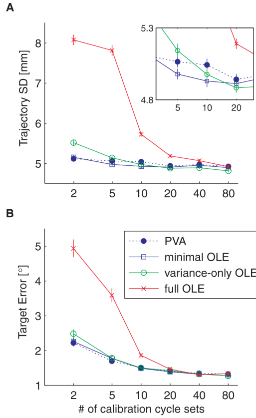
Figure 7. Decoding performance of the different decoders under closed-loop control, for 30 simulated neurons. A. Average trajectory SD ( \pm 1 SE) plotted as a function of the amount of data collected during the calibration session, where a cycle set is one presentation of each of 8 targets spaced uniformly around a circle. The inset shows a close up of the given range. B. Same, for the target angular error.
