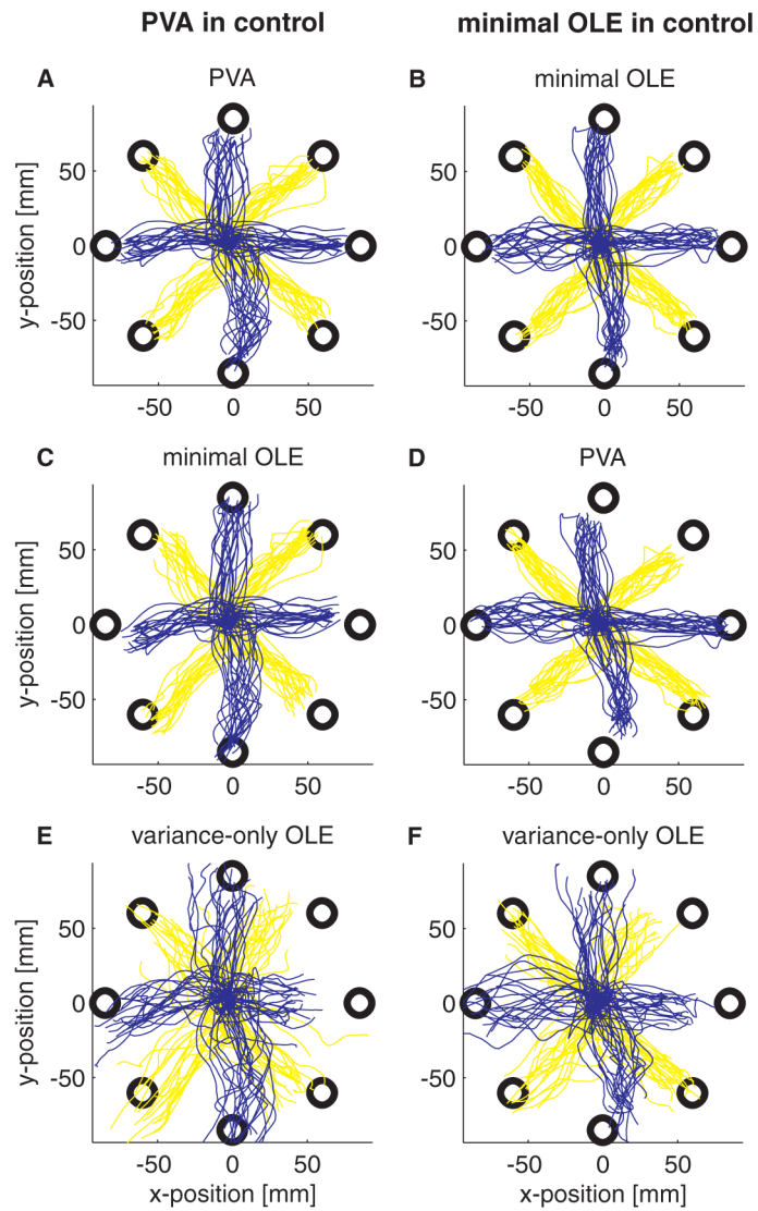
Figure 5. Same as Fig. 4, for an experiment where PVA decoding was compared to minimal OLE decoding. 33 cells drove the cursor in this experiment.
