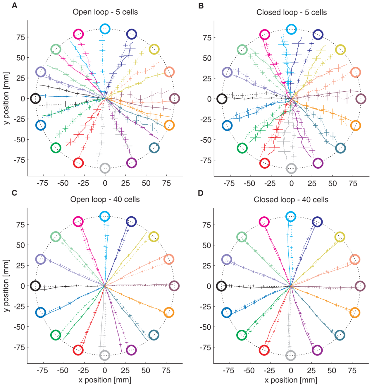
Figure 2. Simulation results. Mean ( \pm 1 SE) of the trajectories to each of the 16 targets. PVA trajectories are shown as solid lines, minimal OLE trajectories as dashed lines. A. Open-loop control using 5 simulated neurons. B. Closed-loop control with the same 5 cells. C. Open-loop control with 40 neurons. D. Closed-loop control with those 40 cells.
