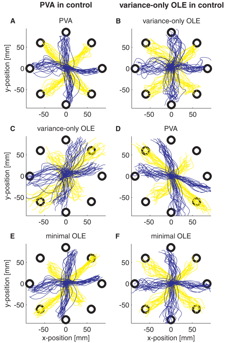
Figure 4. Experimental results comparing PVA decoding (left hand column) to variance-only OLE decoding (right hand column). The same 30 cells were used with each decoder. Color changes across targets are to aid visibility. A. Actual cursor trajectories during PVA control. C, E. Trajectories that result when the spike trains recorded during the PVA-controlled trajectories in A are decoded off-line with the variance-only OLE decoder ( C ) or the minimal OLE decoder ( E ). Essentially, these are the open-loop trajectories that result from OLE decoding of a PVA-controlled system. B. Actual cursor trajectories during variance-only OLE control. D, F. Trajectories that result when the spike trains from the variance-only OLE-controlled trajectories in B are decoded with the PVA decoder ( D ) or the minimal OLE decoder ( F ).
