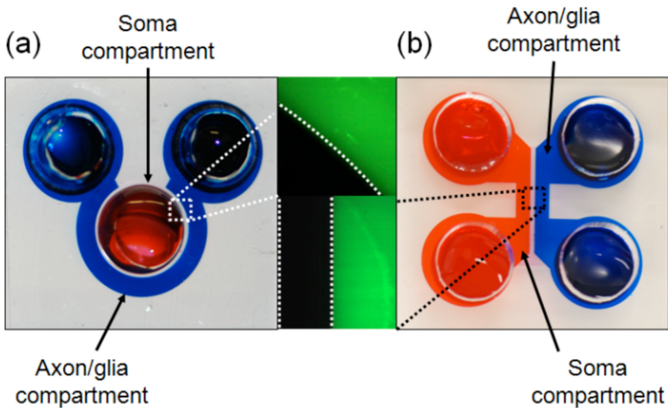
Figure 4. Fluidic isolation in the (a) circular design and (b) square design neuron culture platform. Dotted white lines in the center fluorescence images delineate compartment boundaries. Green fluorescent part indicates the axon/glia compartment while the black part indicates the array of axon-guiding microchannels.
