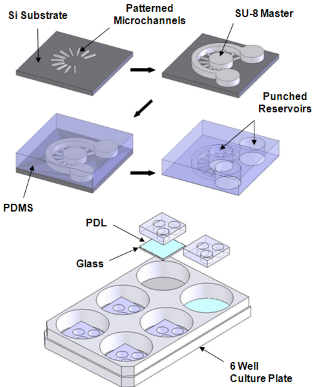
Figure 2. Fabrication and assembly steps for the microfluidic co-culture device. Two SU-8 TM layers with different thicknesses were patterned on top of a silicon substrate to form the axon-guiding microchannel array and the two cell culture compartments (soma, axon/glia). PDMS devices were replicated from the SU-8 master using soft lithography process and 7 mm diameter reservoirs were punched out followed by sterilization in 70% ethanol for 30 minutes and bonding onto PDL or Matrigel TM coated substrates. Each device fits into one well of a conventional 6-well polystyrene culture plate.
