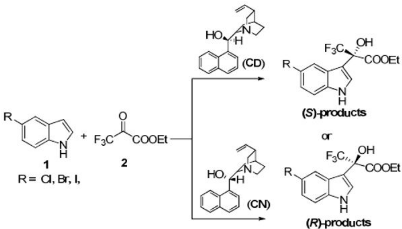
Figure 2. Schematic synthesis of the chiral inhibitors.
